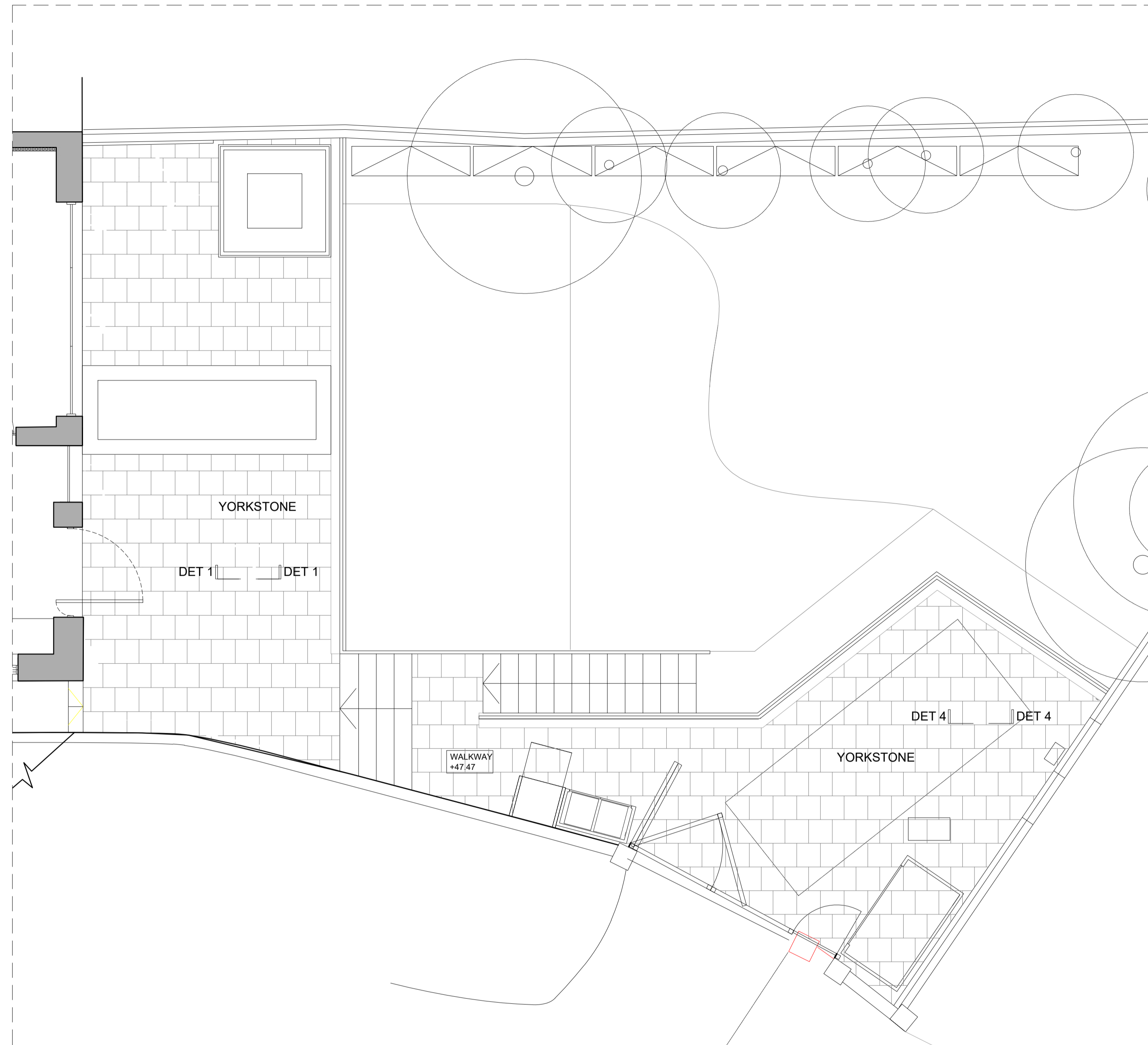
LOWER GROUND FLOOR LEVEL PLAN- TERRACE
