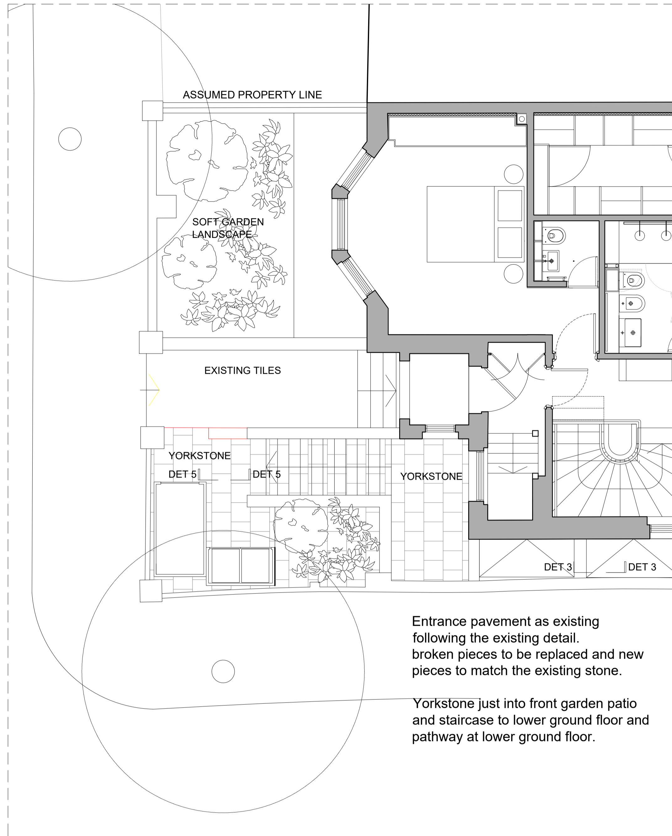
GROUND FLOOR LEVEL PLAN- ENTRANCE
