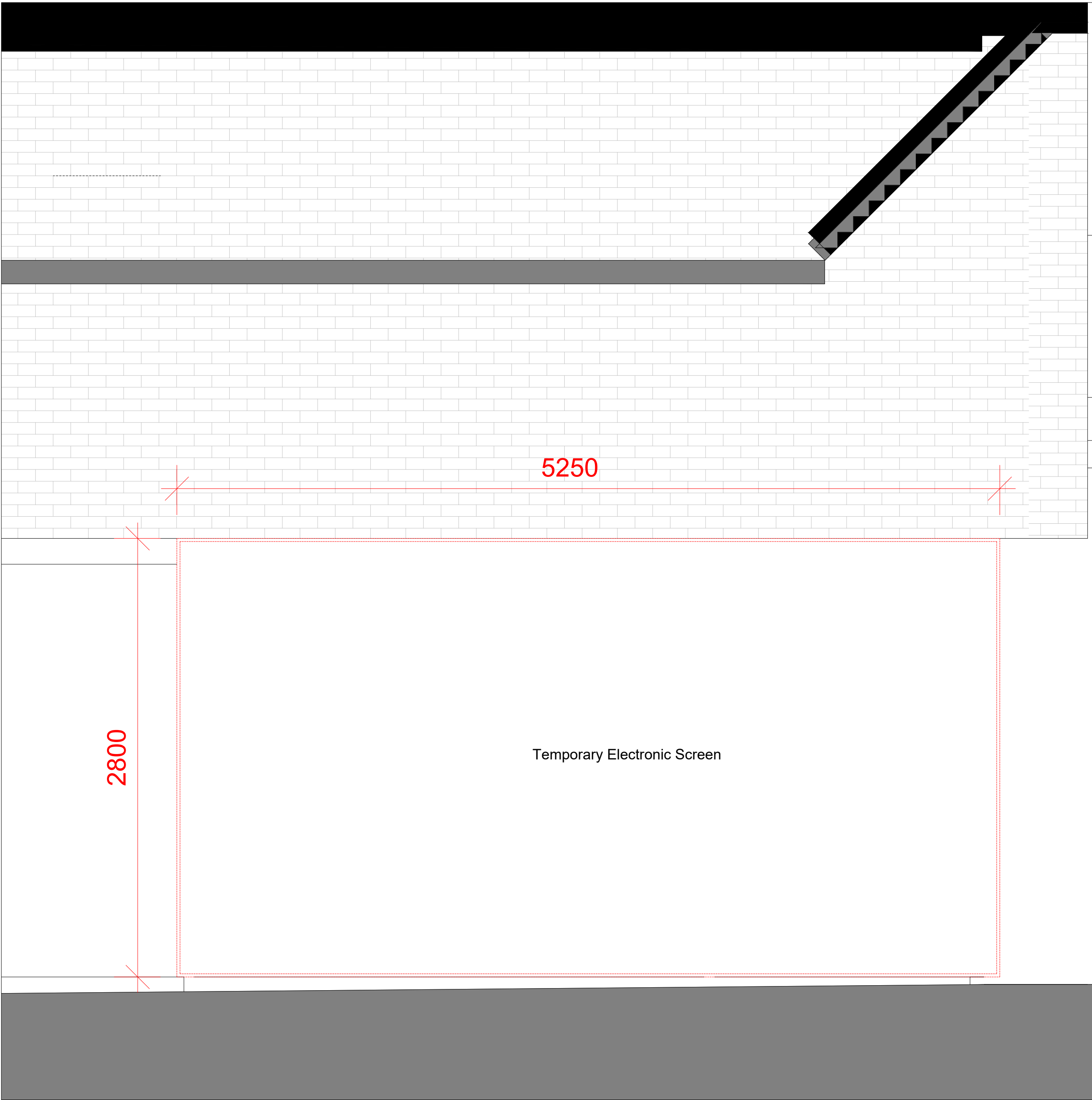
2 C1 CUT-THROUGH ELEVATION (Courtyard side)
