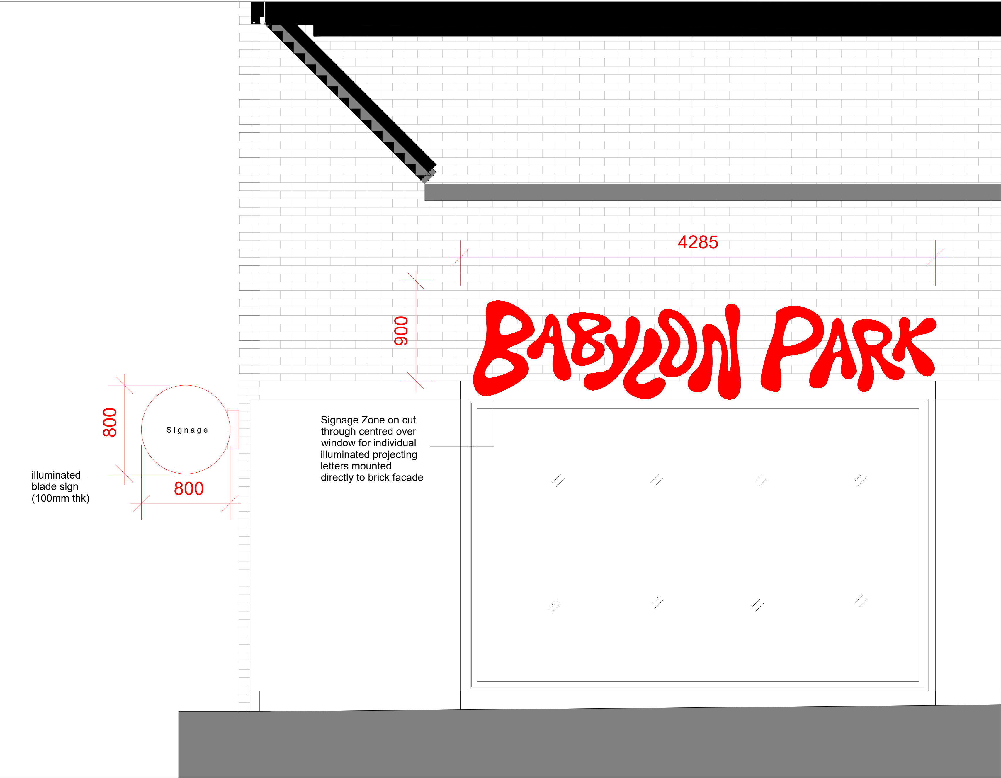
1 C1 CUT-THROUGH ELEVATION (Castlehaven road side)
