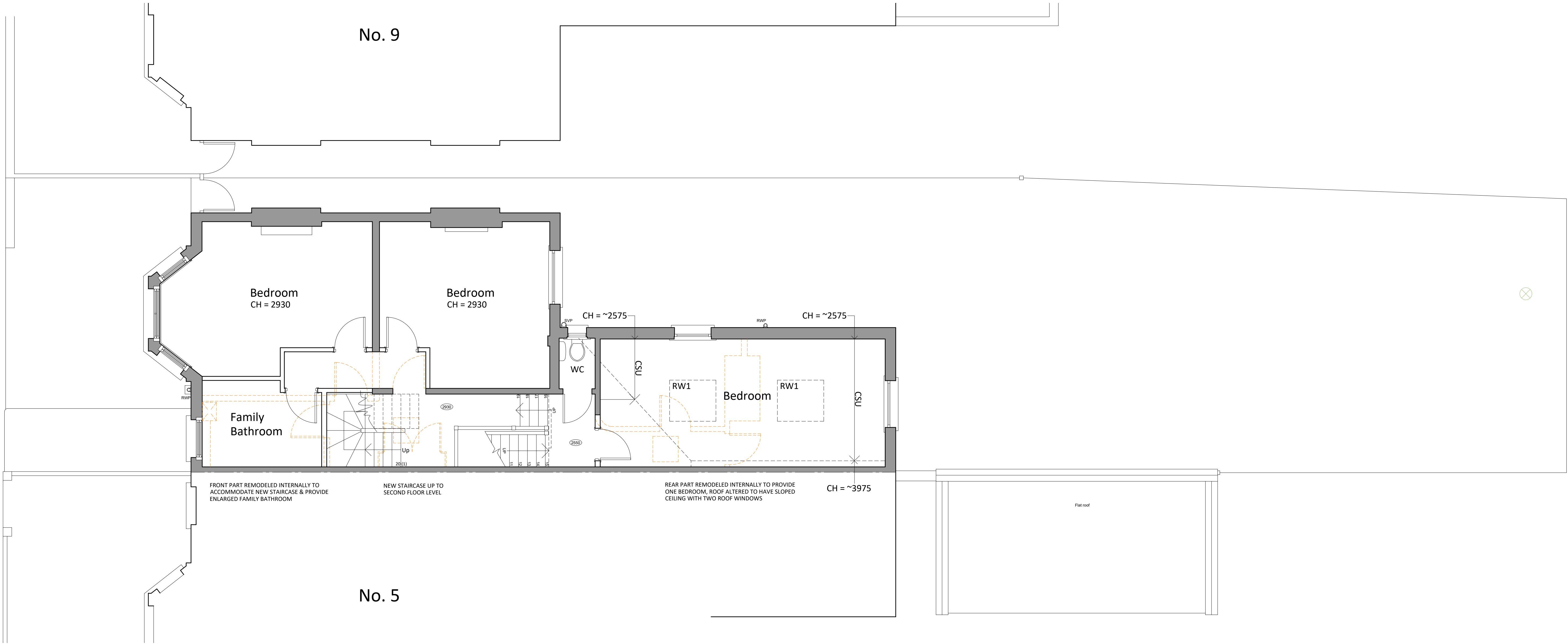
Proposed First Floor Plan 1:50 Scale
