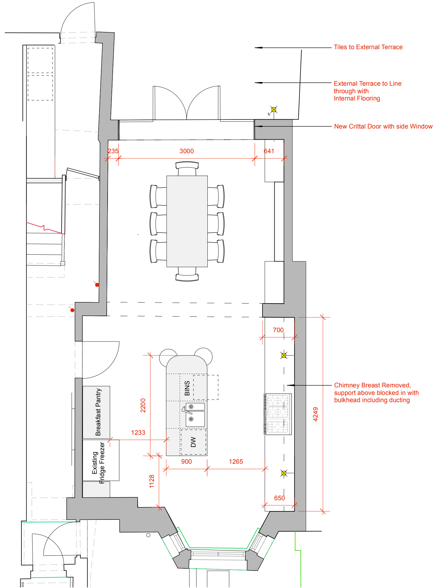
1 Proposed LGF Plan Scale: 1:50
