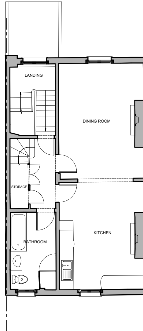
02 SECOND FLOOR PLAN AS EXISTING
