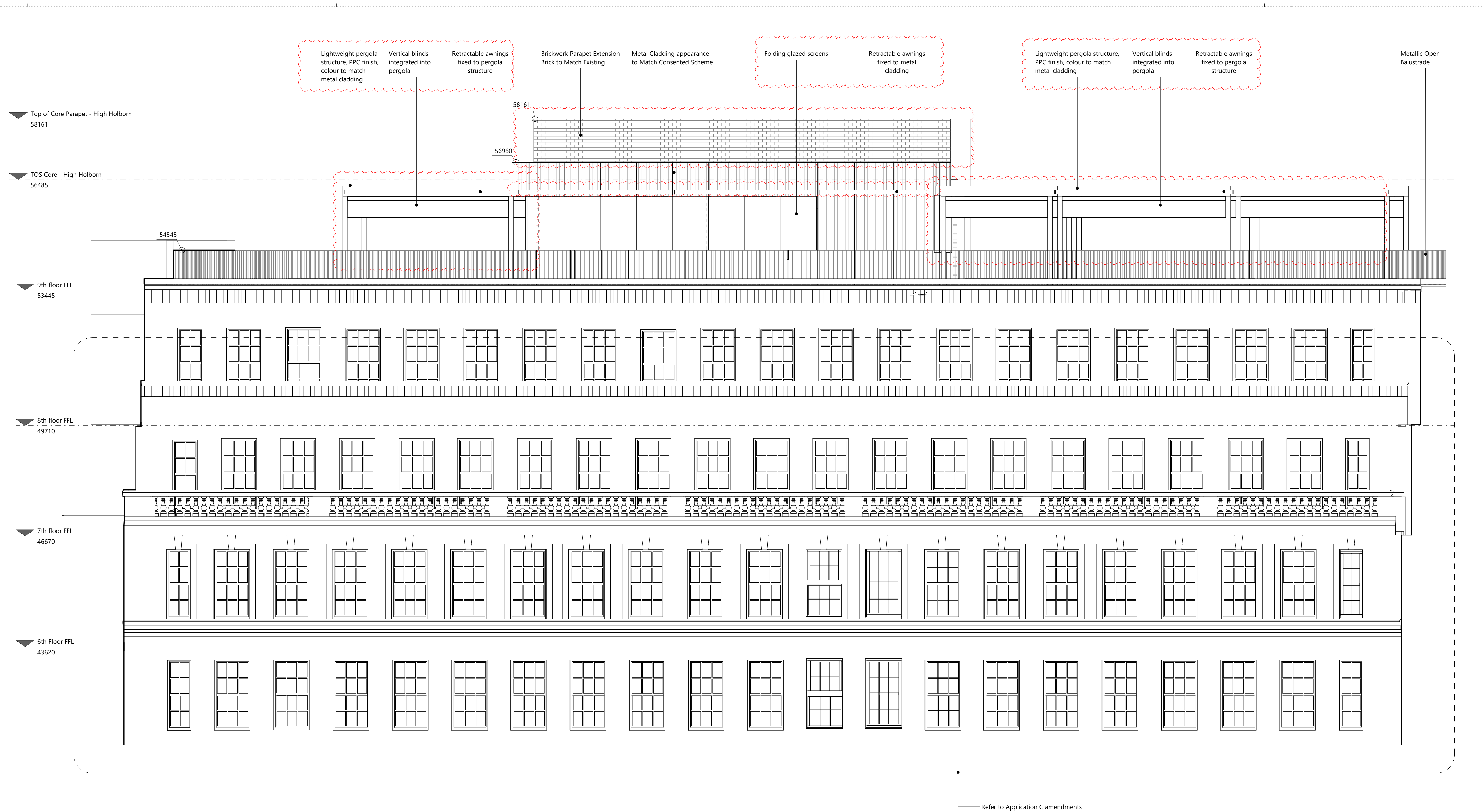
1 South Elevation 1:50
