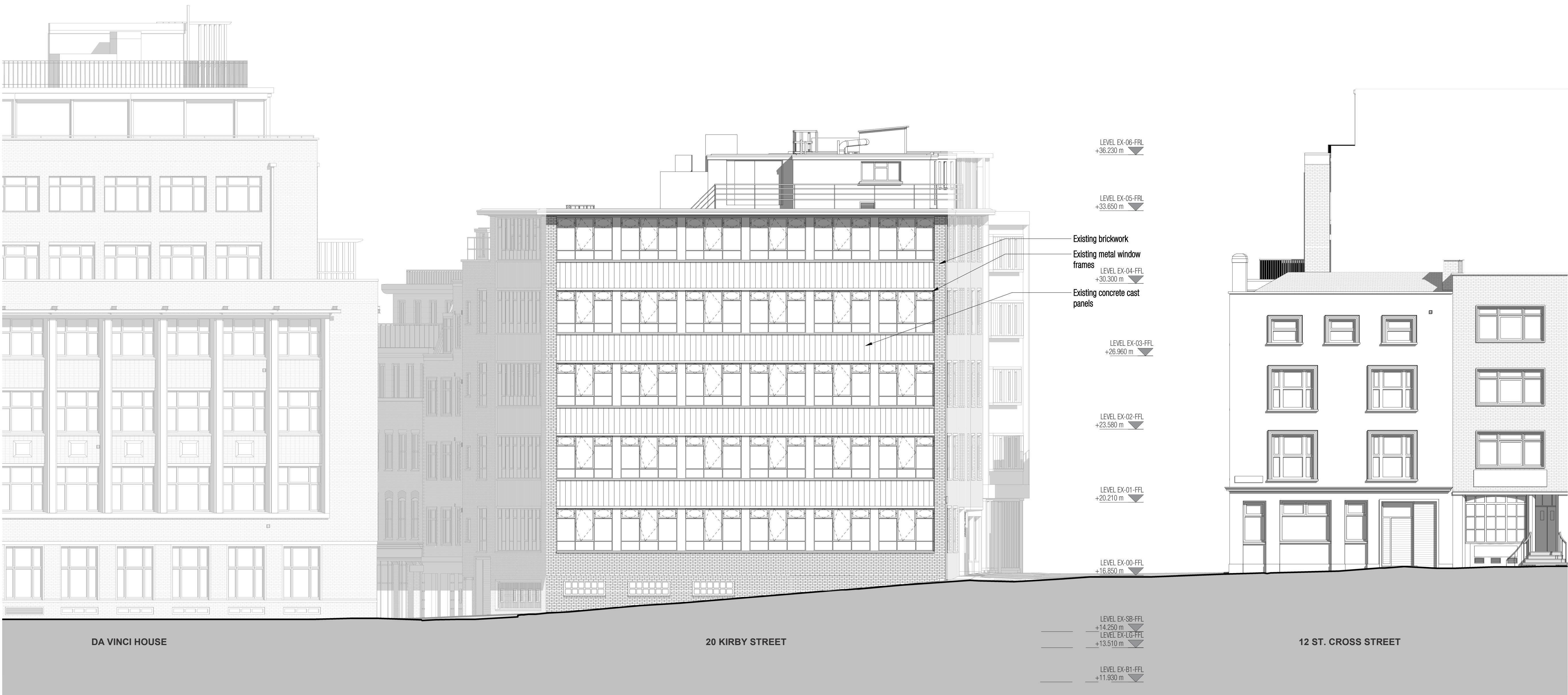
Existing North Elevation
