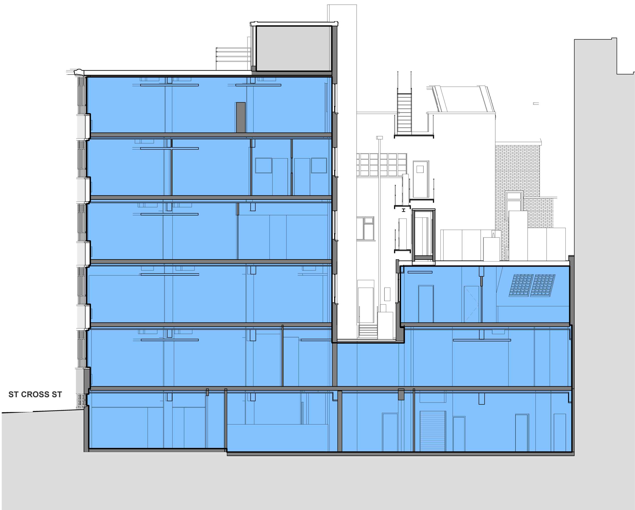
Section BB - Existing
