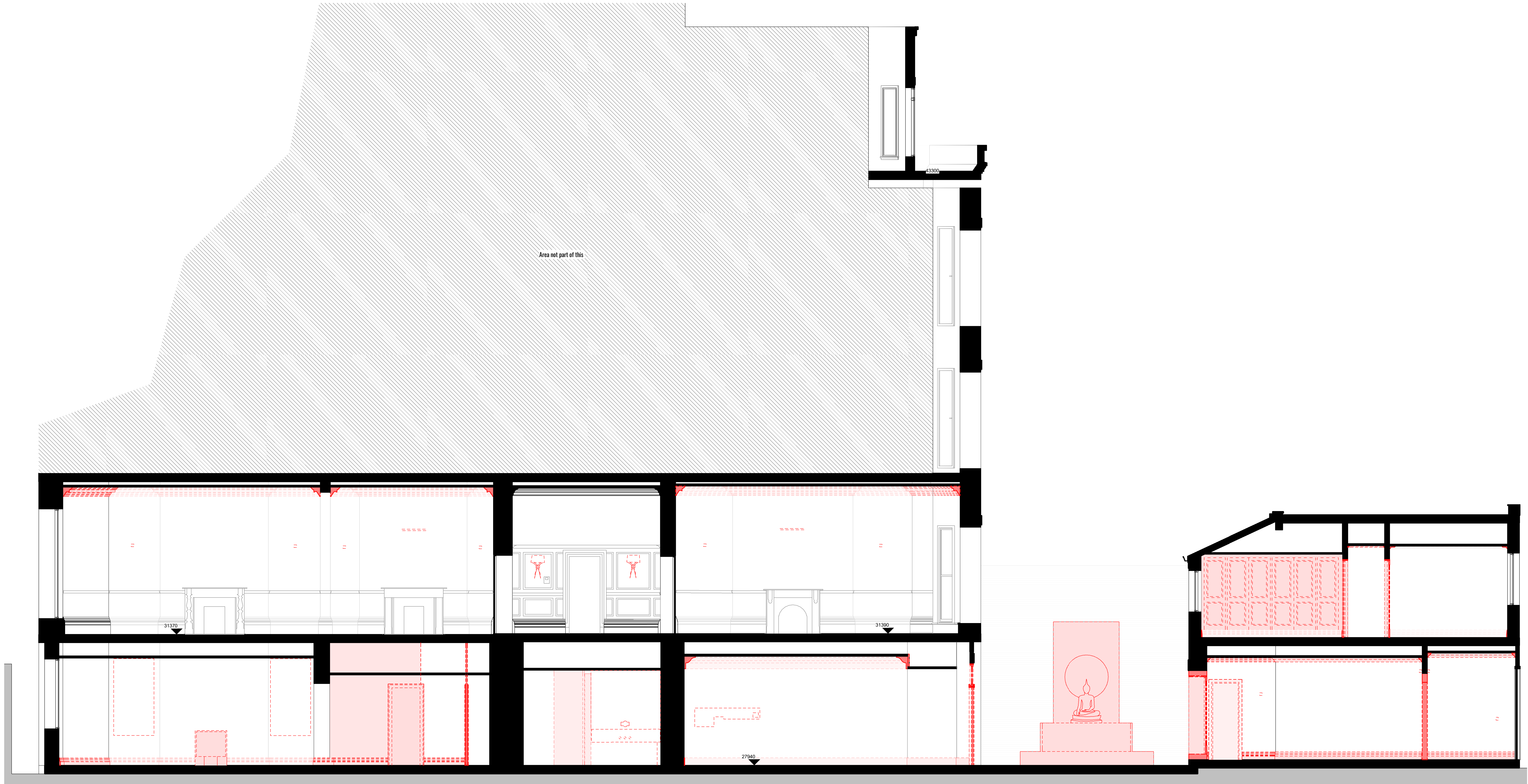
Demolition Section A-A
