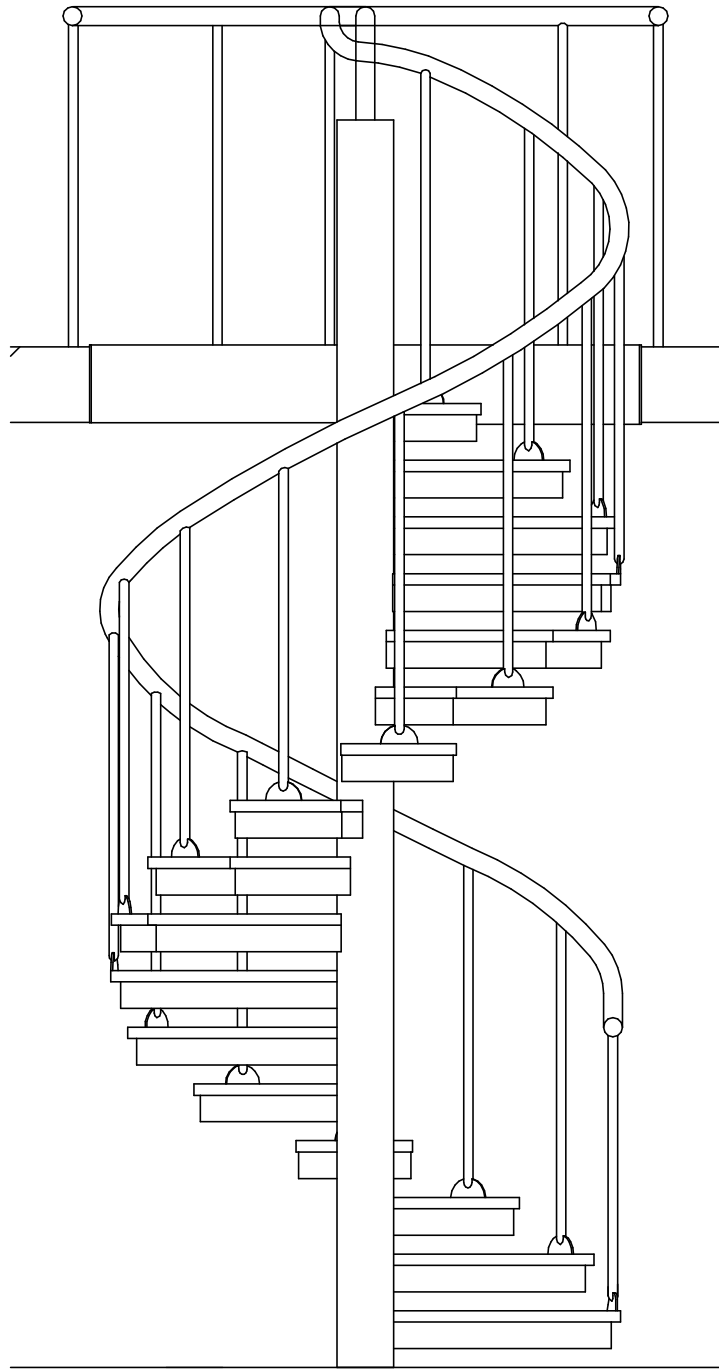
2 Proposed Spiral Stair Elevation
