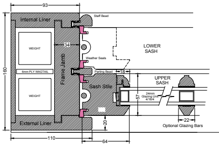
Typical Jamb (Plan) Detail B-B
