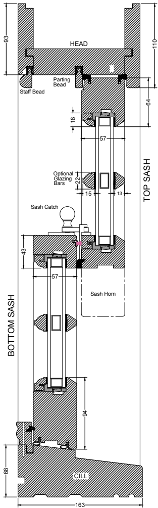
Typical Cill, meeting rail and head detail (Section) Detail A-A
