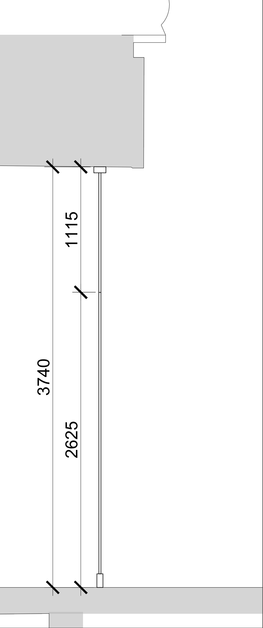
EXISTING SECTION THROUGH SHOPFRONT
