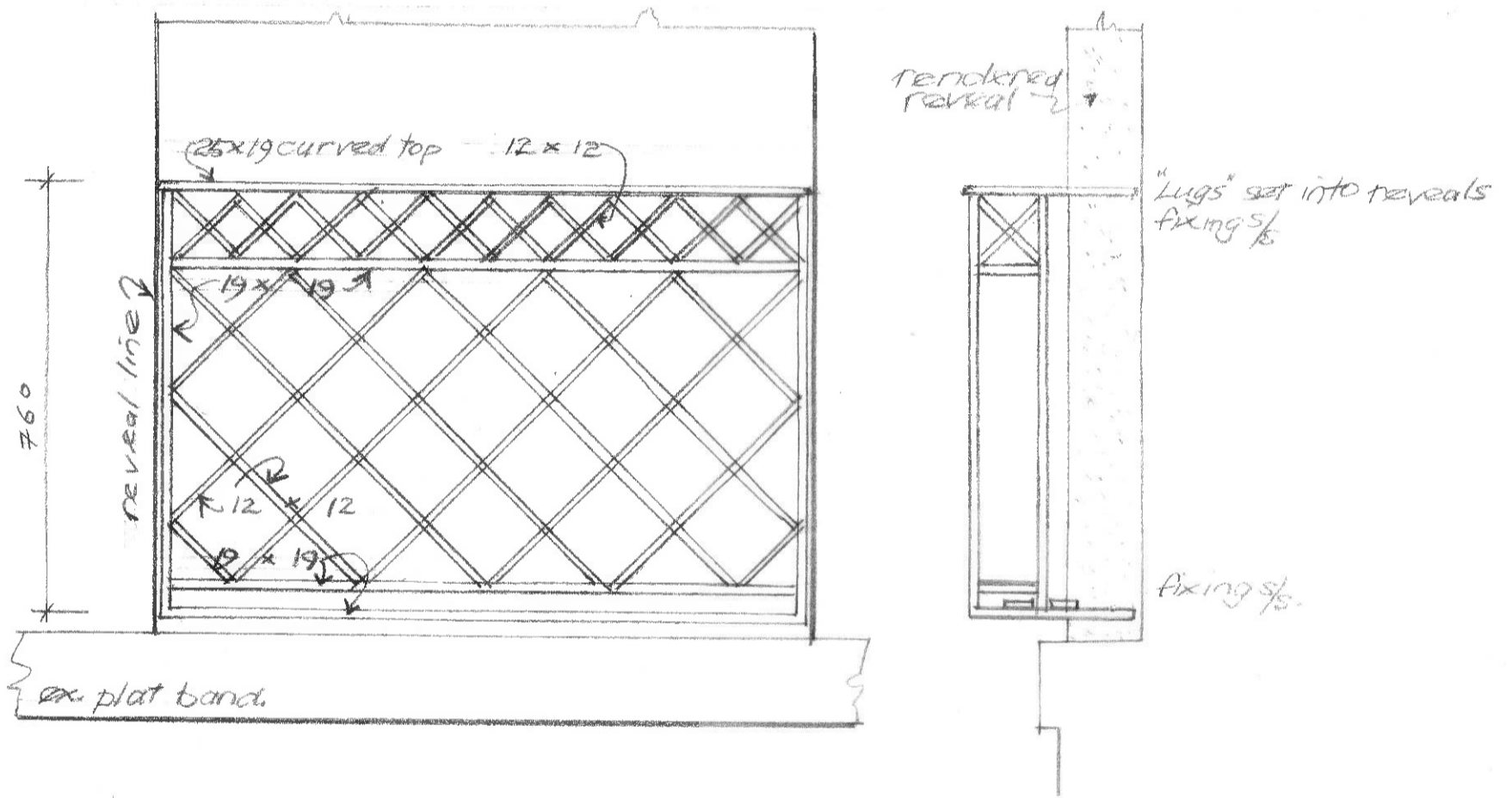
Window Boxes, First Floor, 1:10 @ A3.
