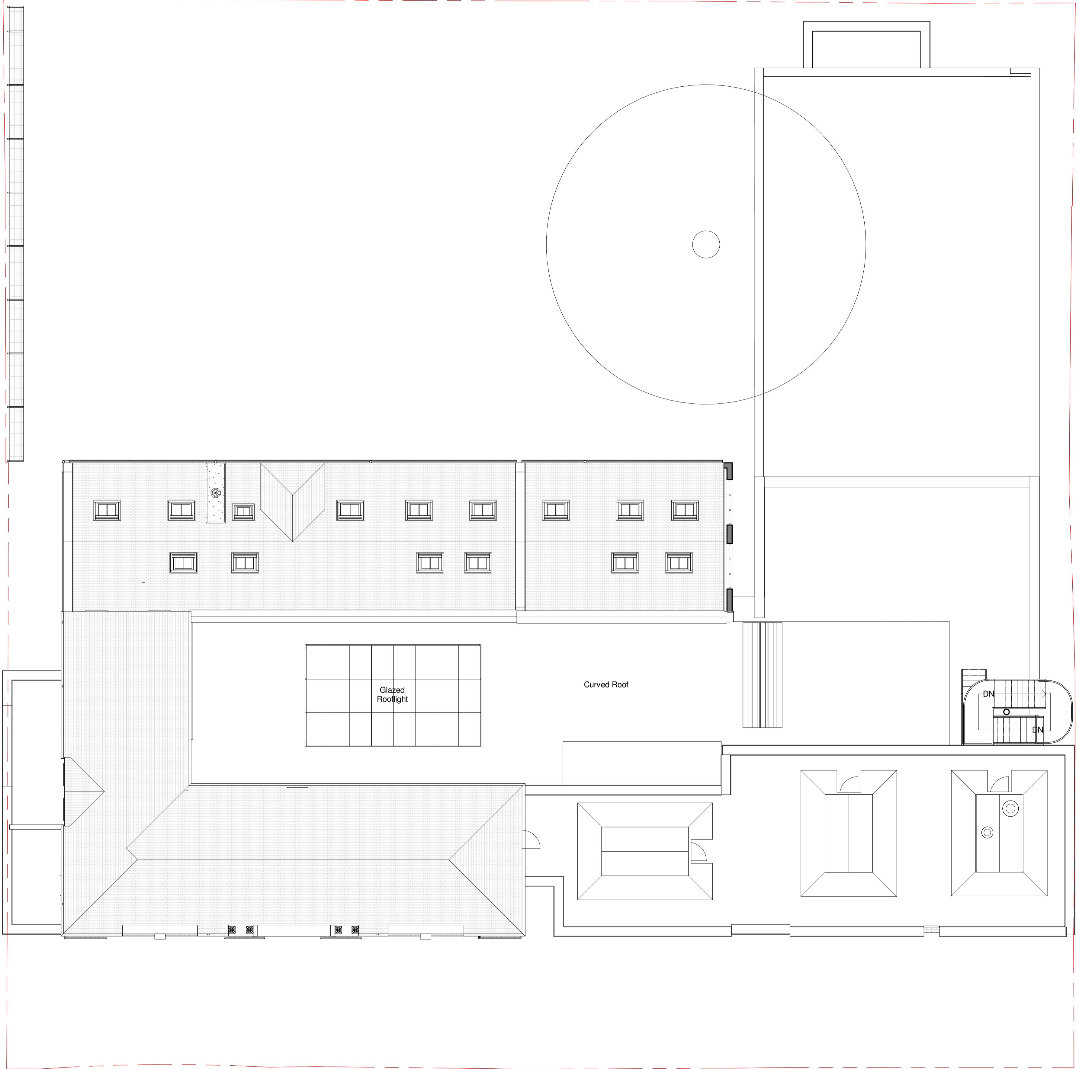
EXISTING GA - ROOF
