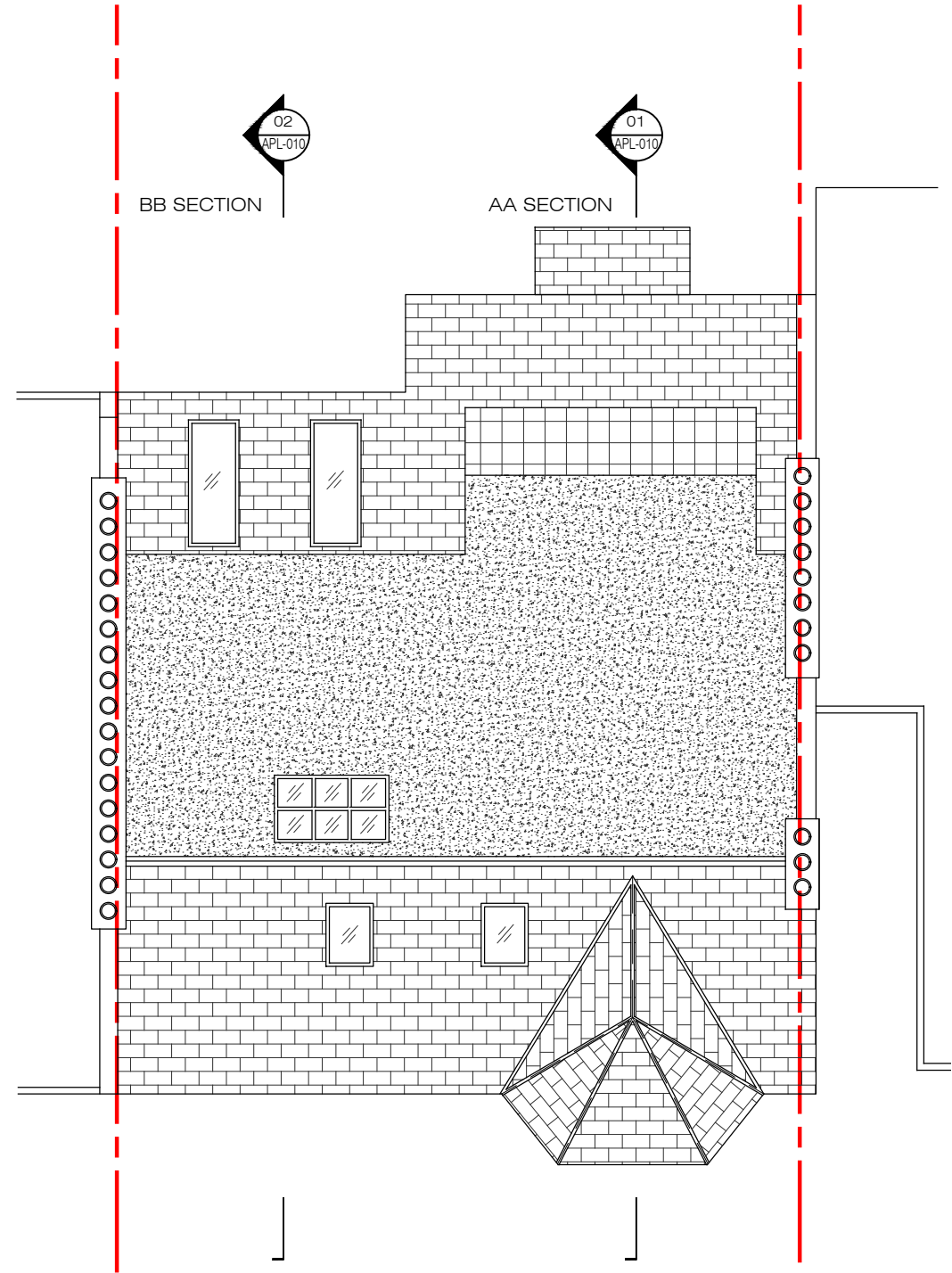
01 Roof Plan scale: 1:100
