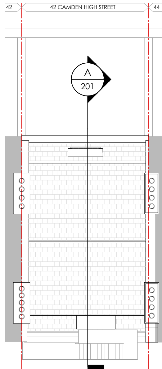
2 ROOF PLAN EXISTING 1:100
