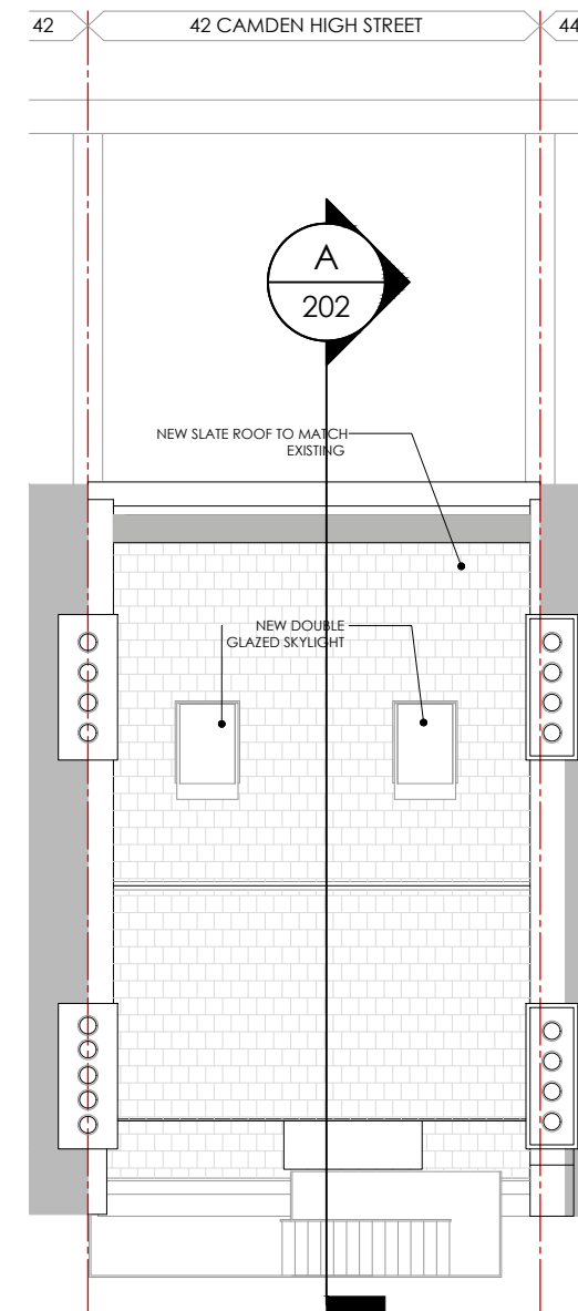
4 ROOF PLAN PROPOSED 1:100
