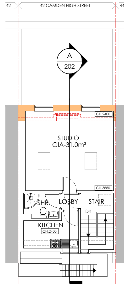
3 THIRD FLOOR PLAN PROPOSED 1:100
