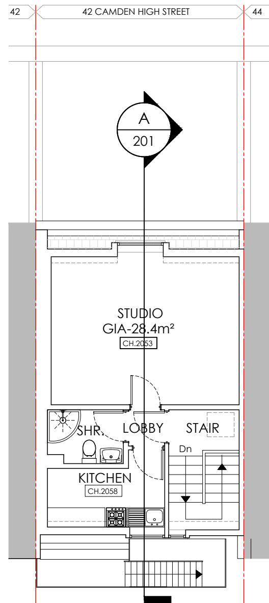
1 THIRD FLOOR PLAN EXISTING 1:100
