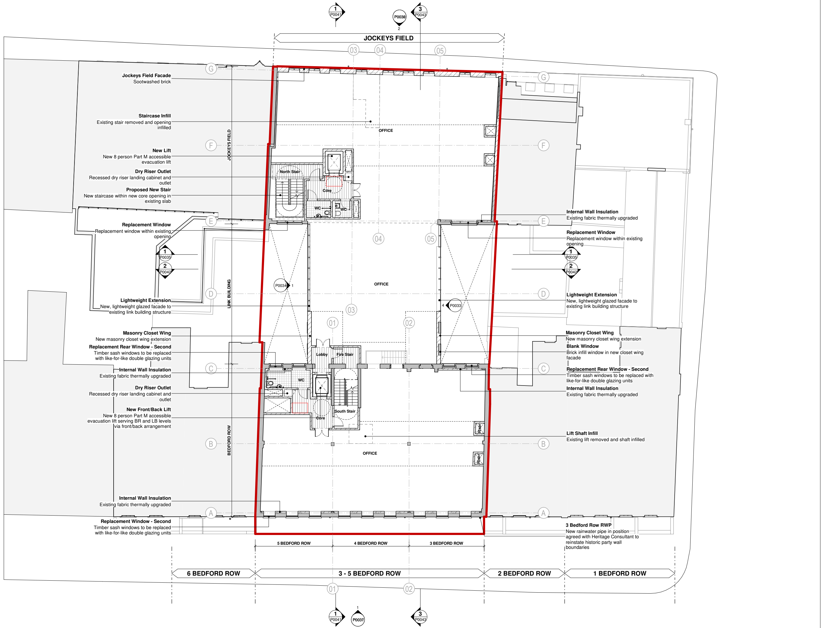
P0012 - D - Proposed Second Floor
