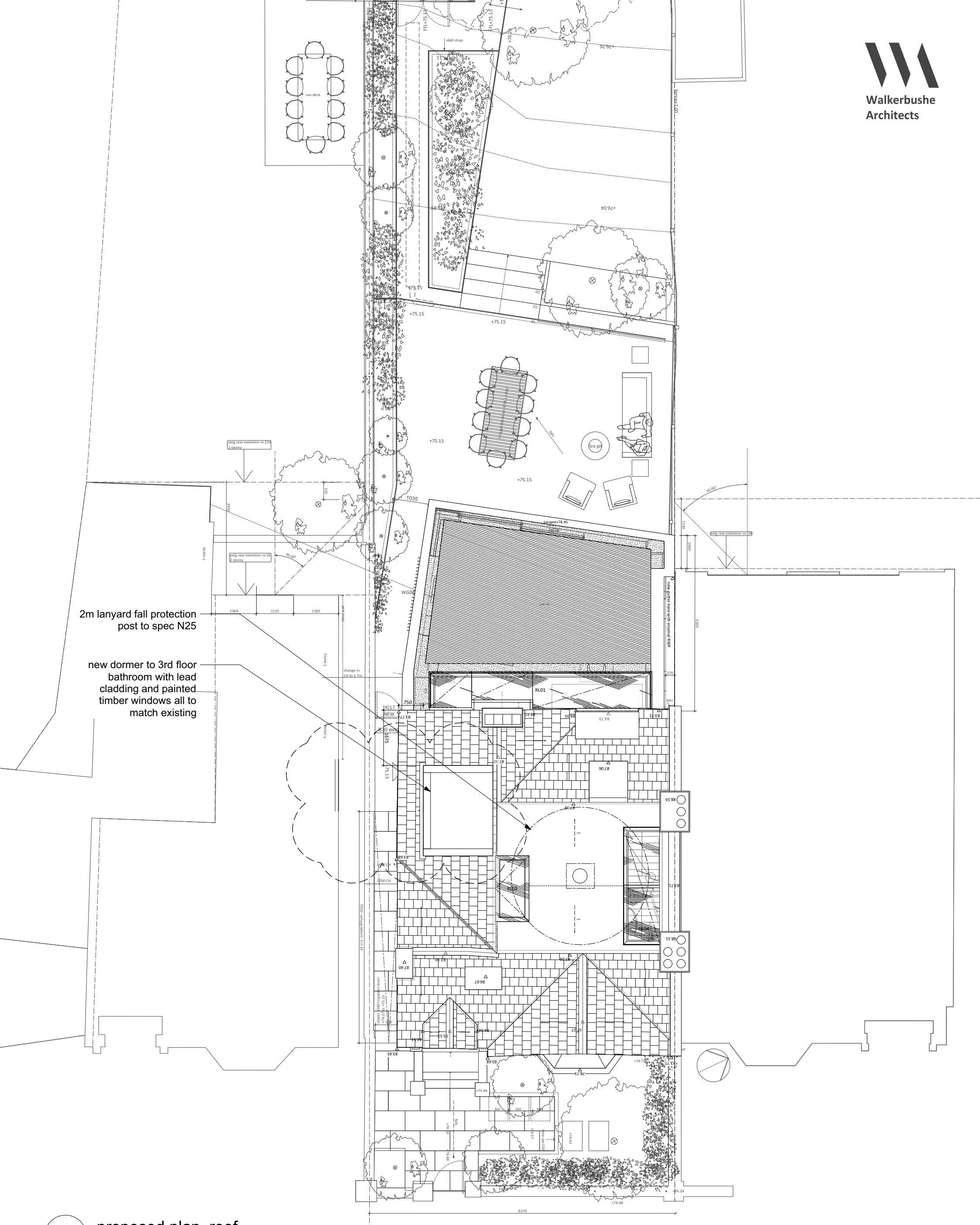
1 proposed plan_roof Scale: 1:100
