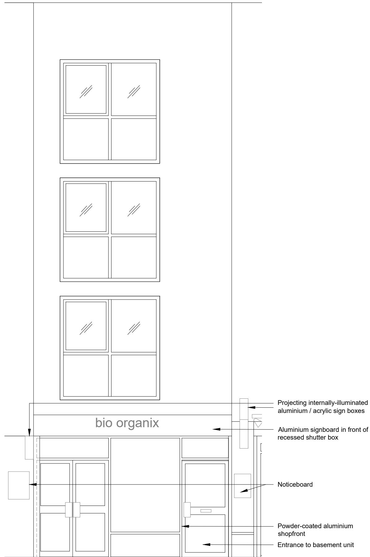
01 Existing Elevation
