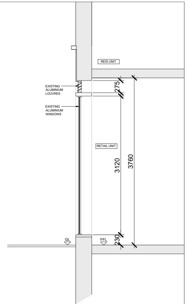
EXISTING SECTION THROUGH SHOPFRONT
