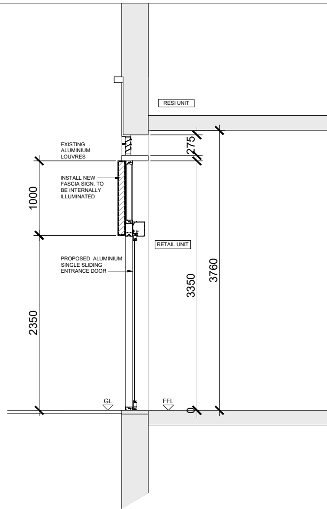
PROPOSED SECTION THROUGH ENTRANCE
