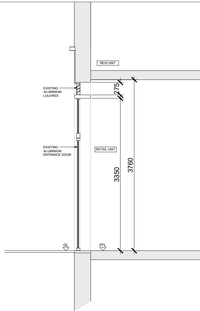
EXISTING SECTION THROUGH ENTRANCE
