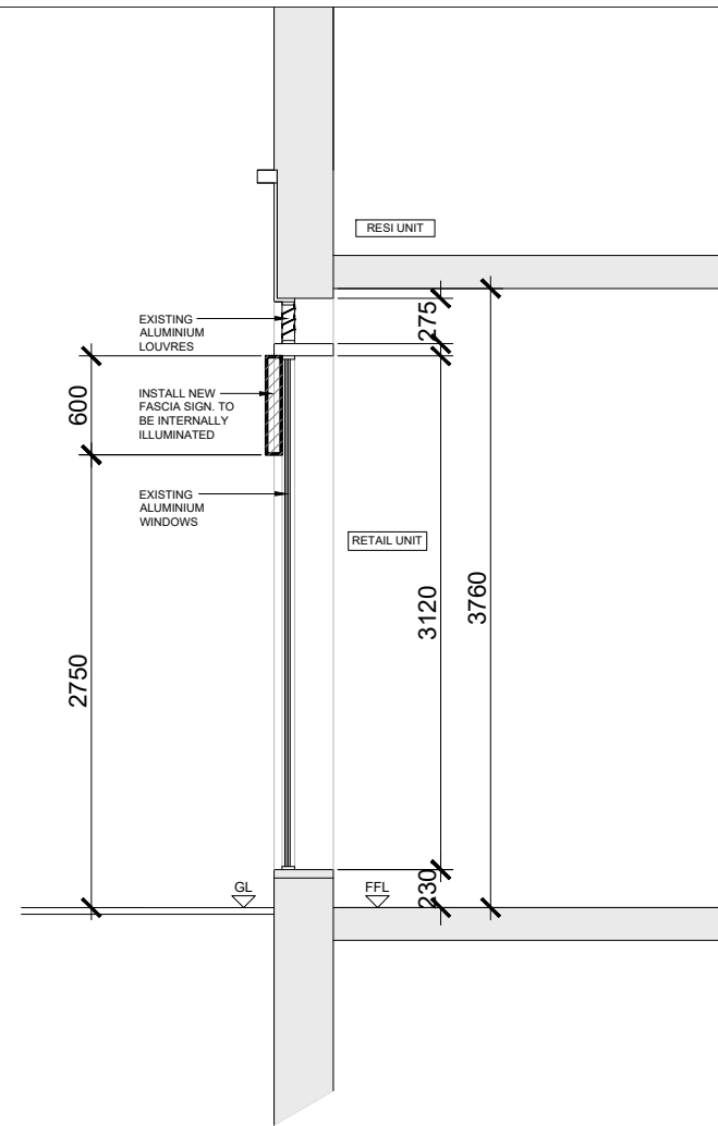
PROPOSED SECTION THROUGH SHOPFRONT
