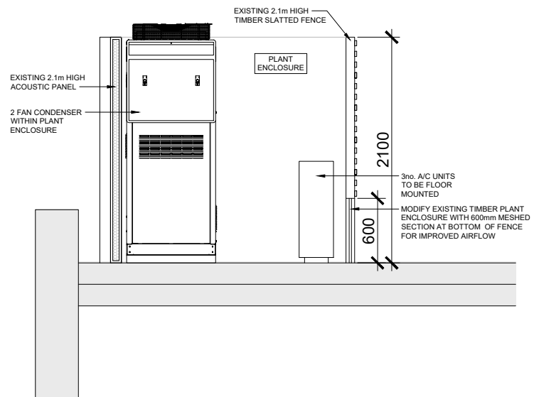
PROPOSED SECTION THROUGH PLANT ENCLOSURE
