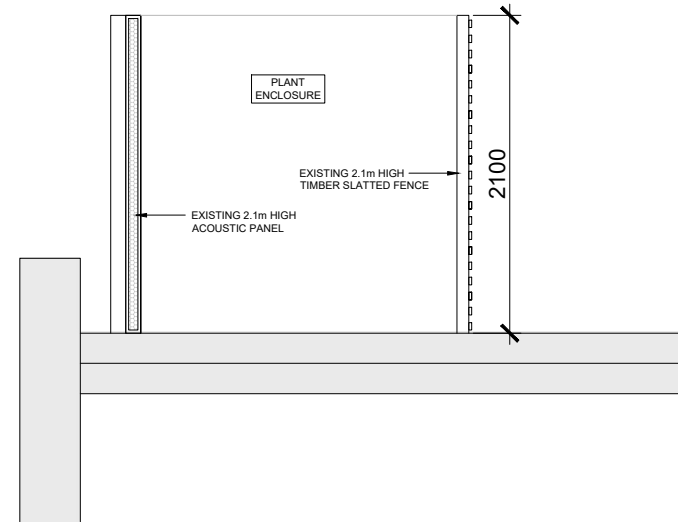
EXISTING SECTION THROUGH PLANT ENCLOSURE
