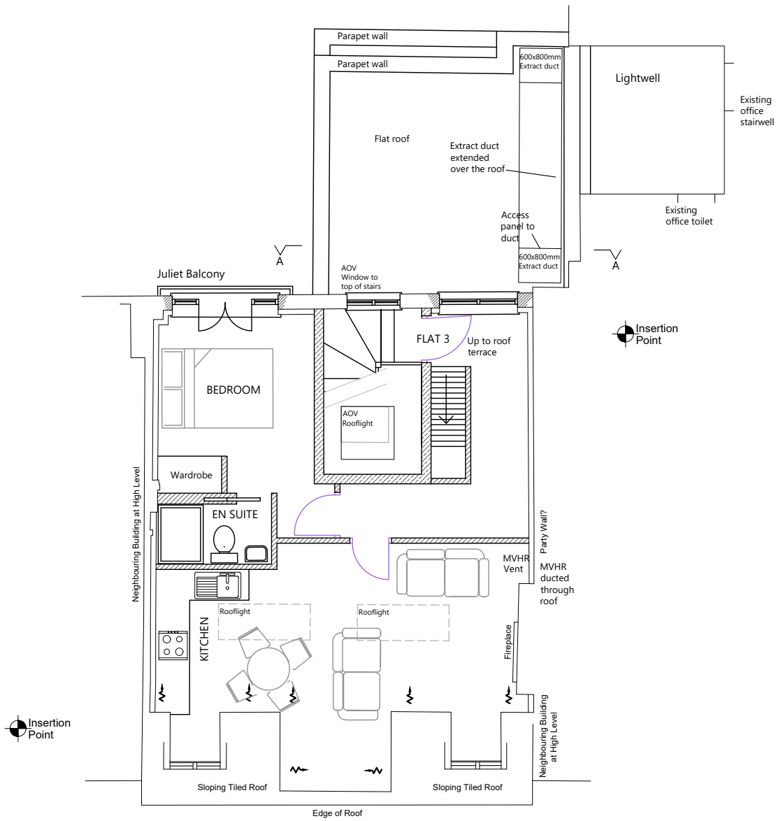
THIRD FLOOR One Bedroom Flat Floor area 51.3sq.m
