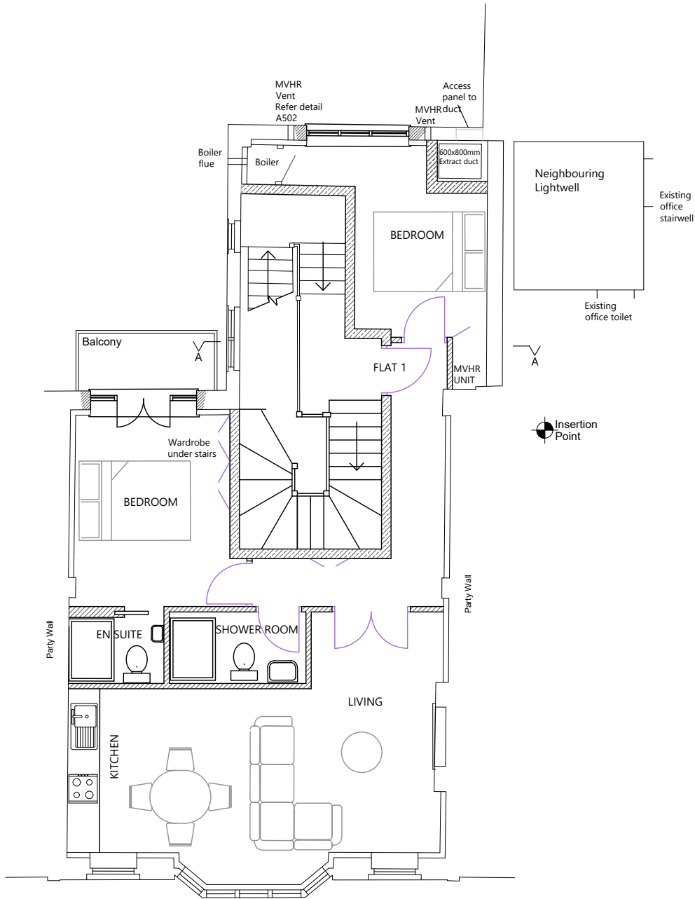
FIRST FLOOR Two Bedroom Flat Floor area 65.8sq.m
