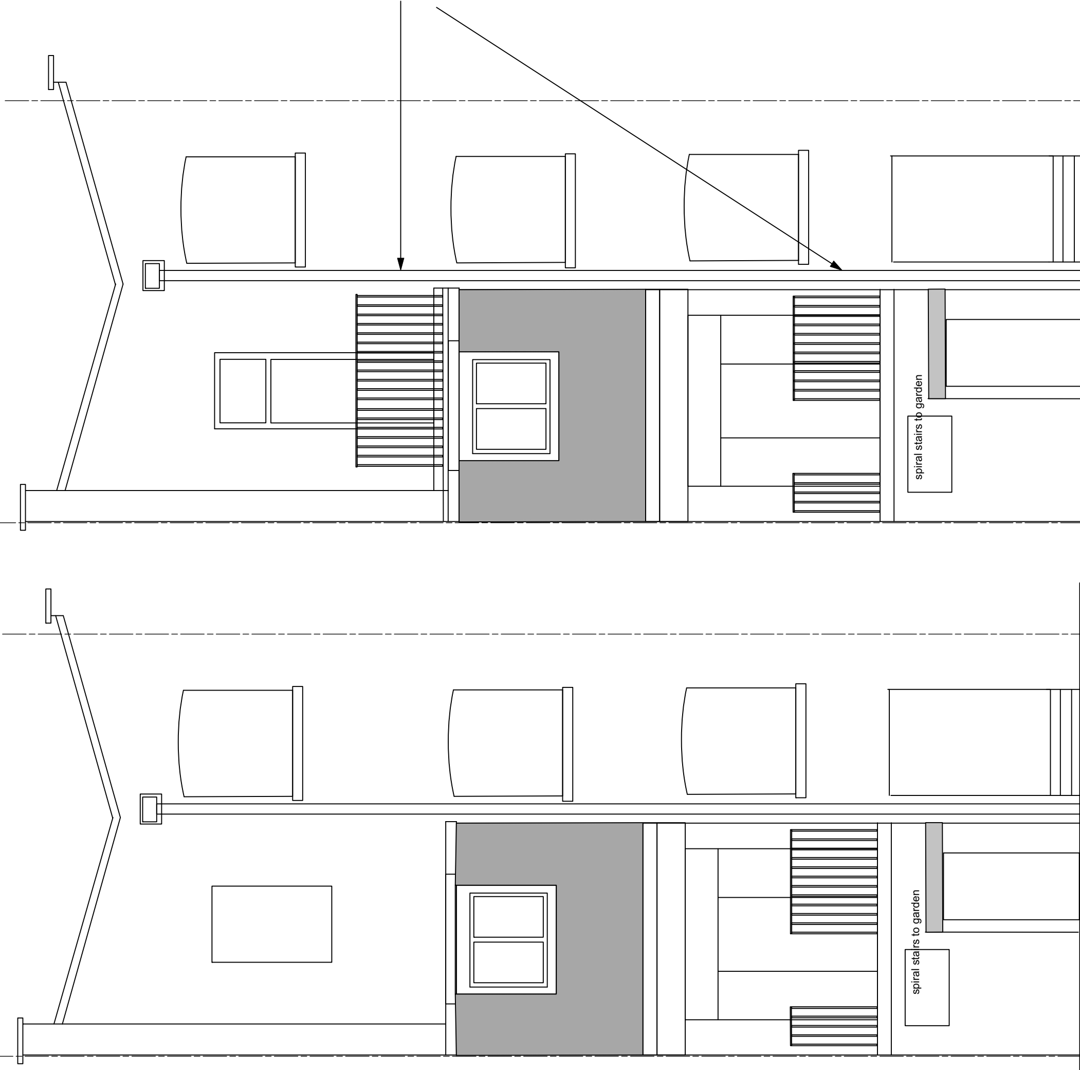
Cast iron decorative railings to existing ground floor balcony and spiral staircase to garden to be replicated on the proposed 1st/2nd floor roof terrace.
