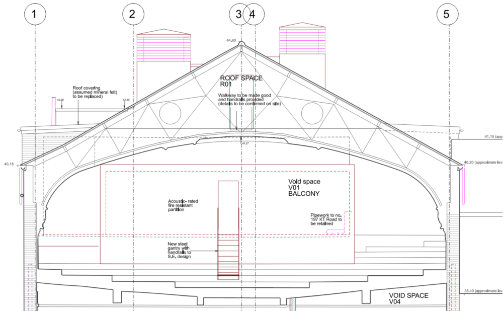
Figure 5 Section view of proposed chiller exhaust vents
