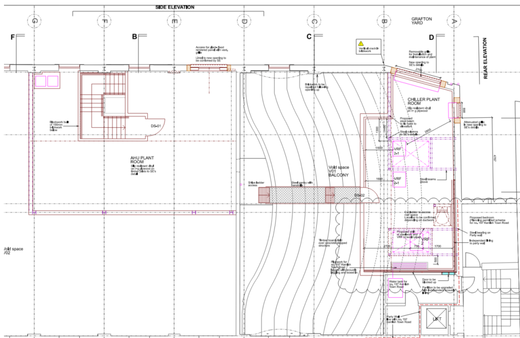
Figure 6 Plan of proposed plant room locations and atmospheric terminations
