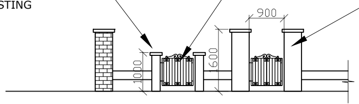
PROPOSED FRONT WALL ELEVATION
