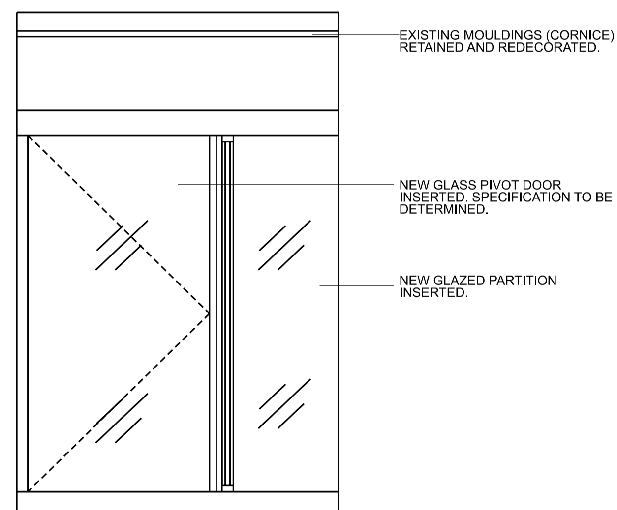
3 1:25@ A1 PROPOSED SOUTH ELEVATION
