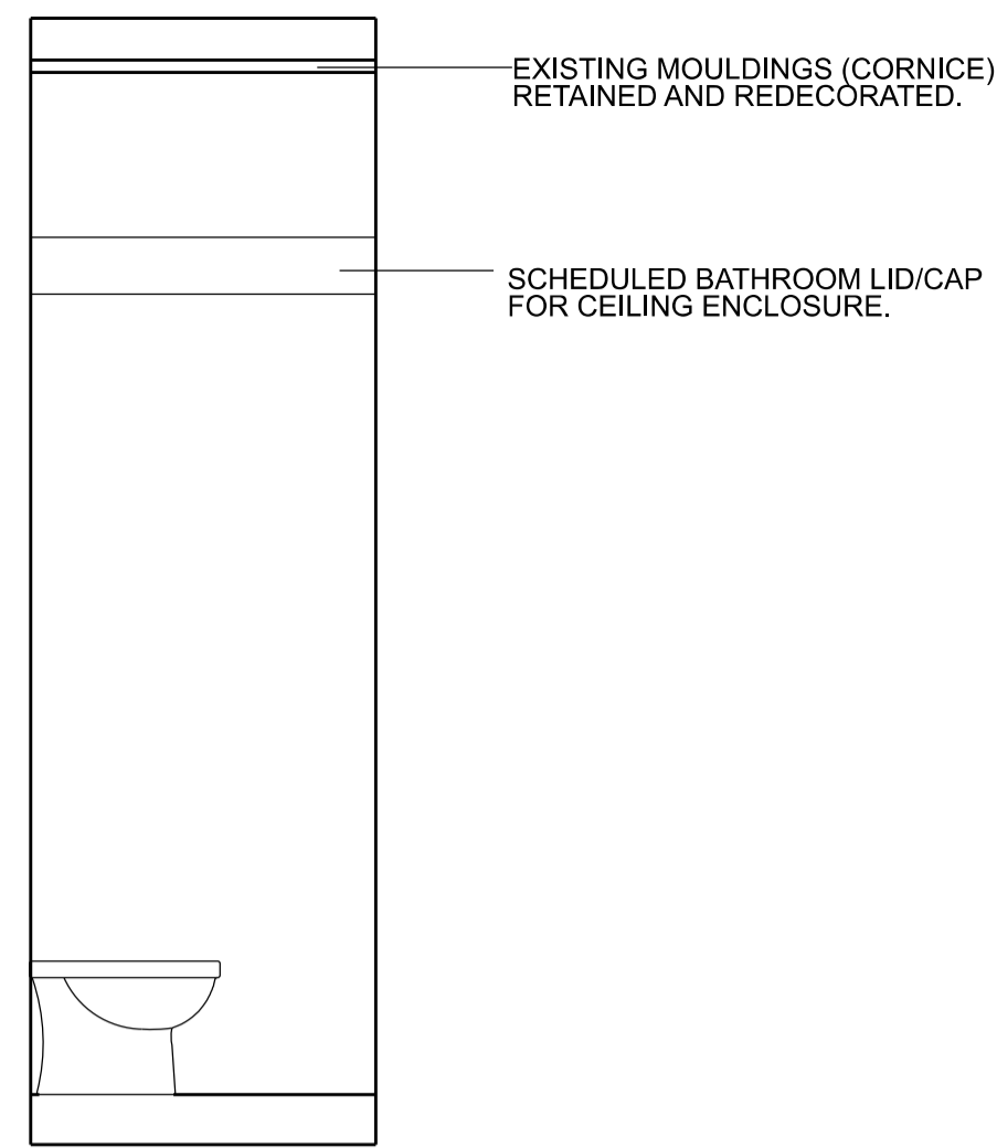
2 1:25@ A1 PROPOSED EAST ELEVATION
