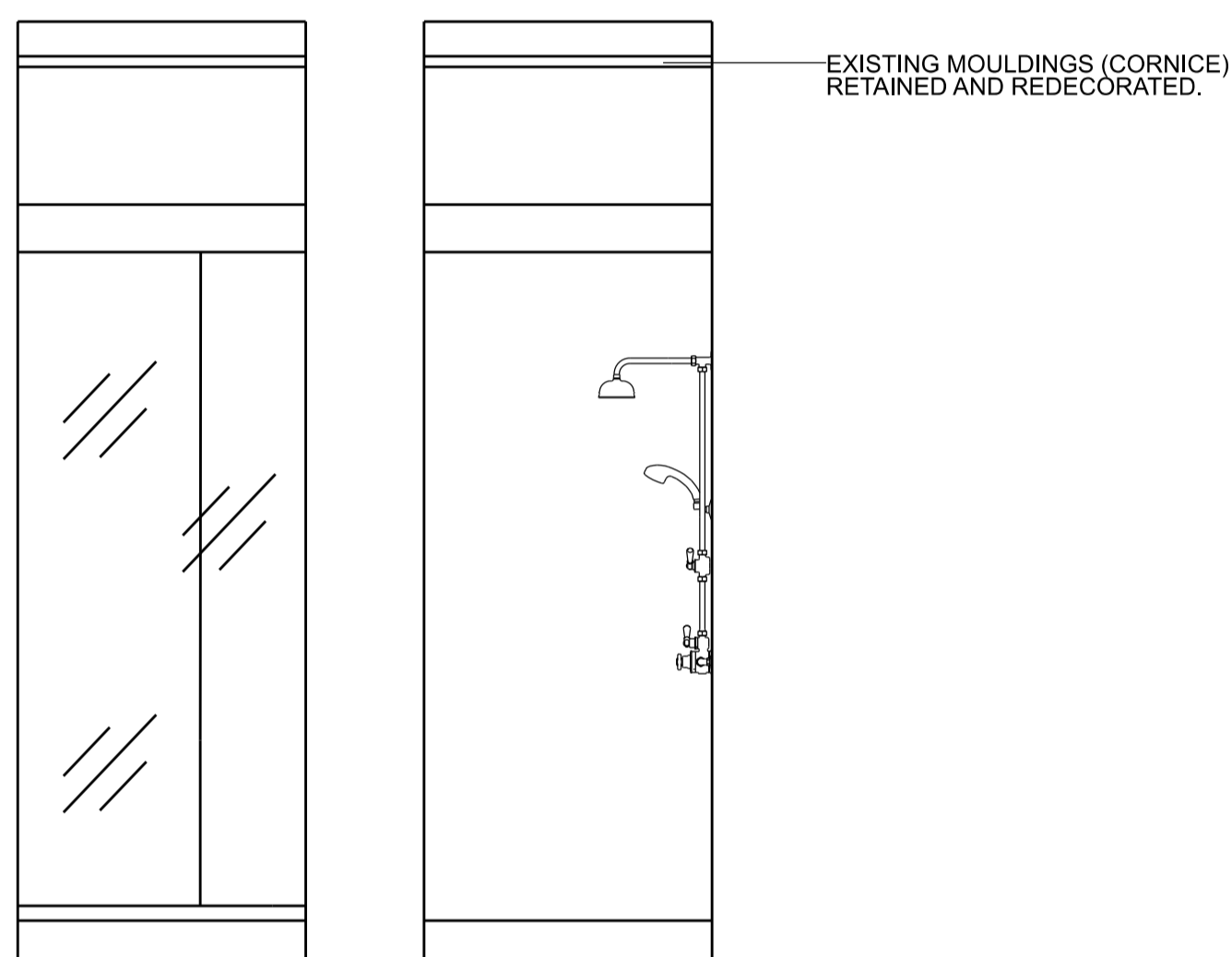
4 1:25@ A1 PROPOSED WEST ELEVATION
