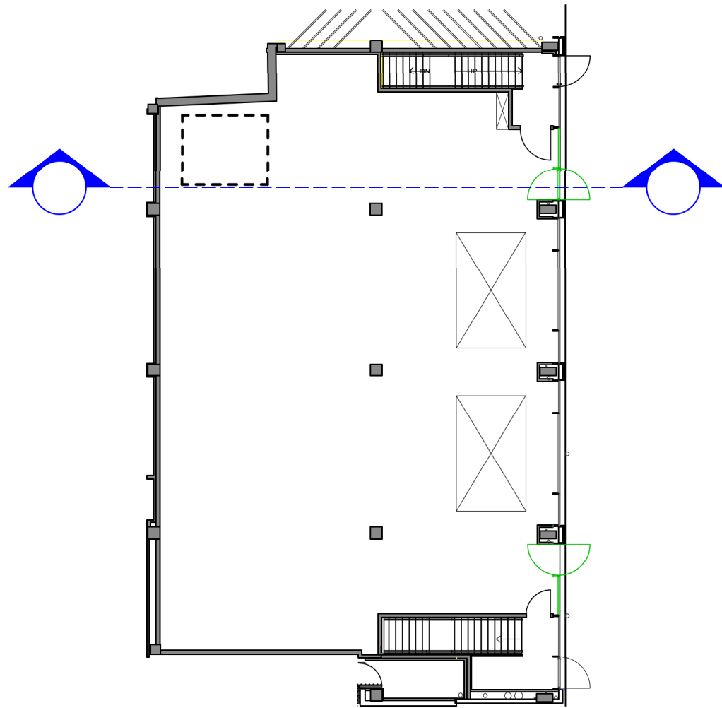
KEY PLAN
