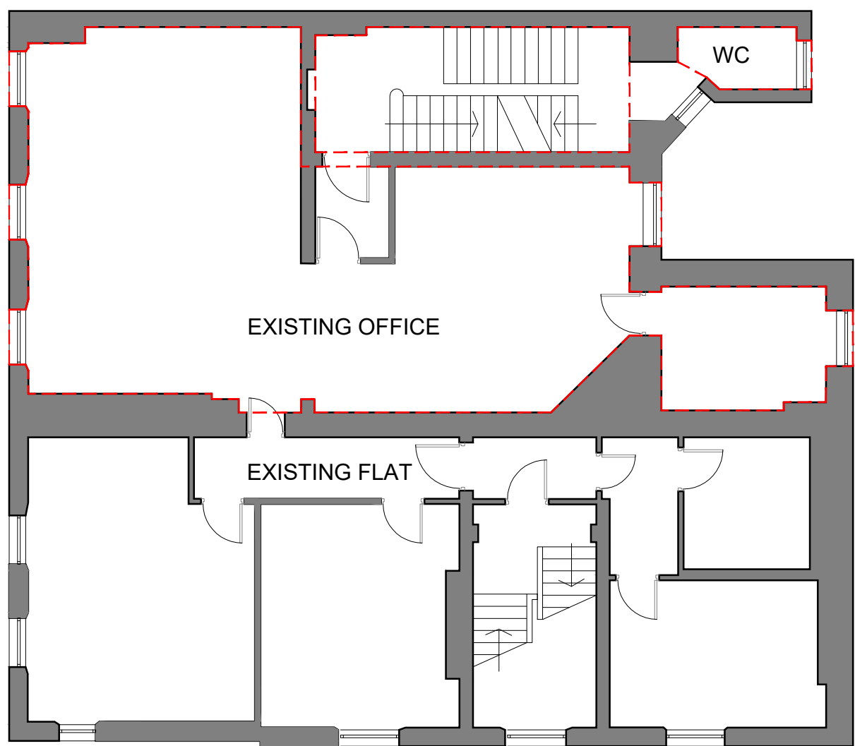
01- EXISTING FIRST FLOOR PLAN
