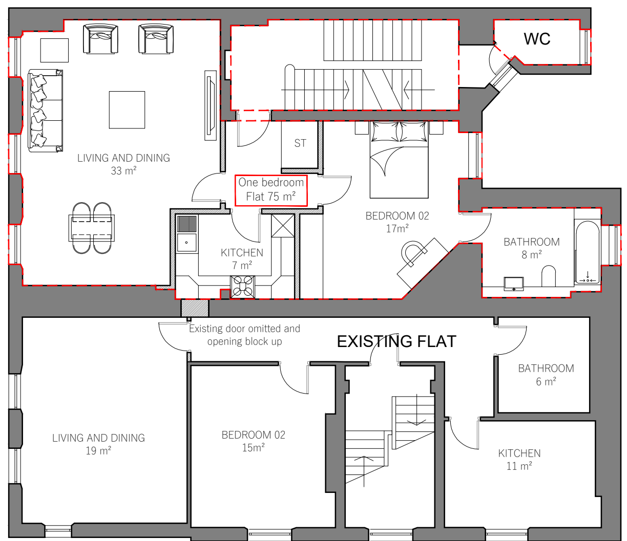
02- PROPOSED FIRST FLOOR PLAN
