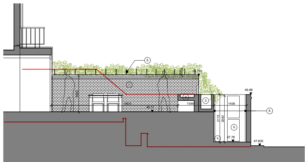
03 - Section/ Elevation - Proposed
