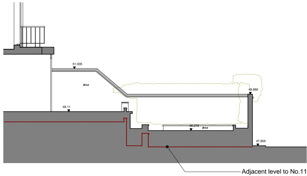
01 - Section/ Elevation- Existing
