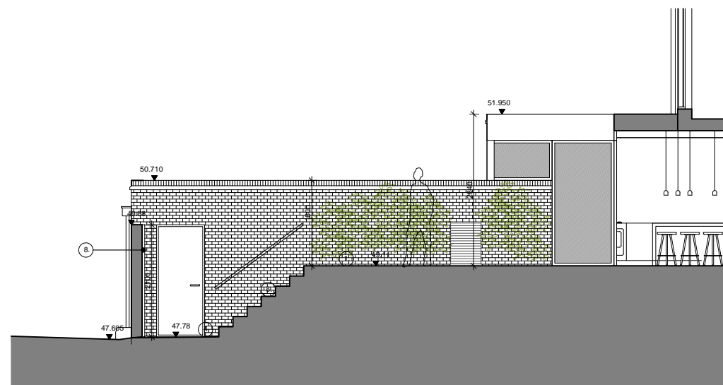
04 - Section/ Elevation - Proposed
