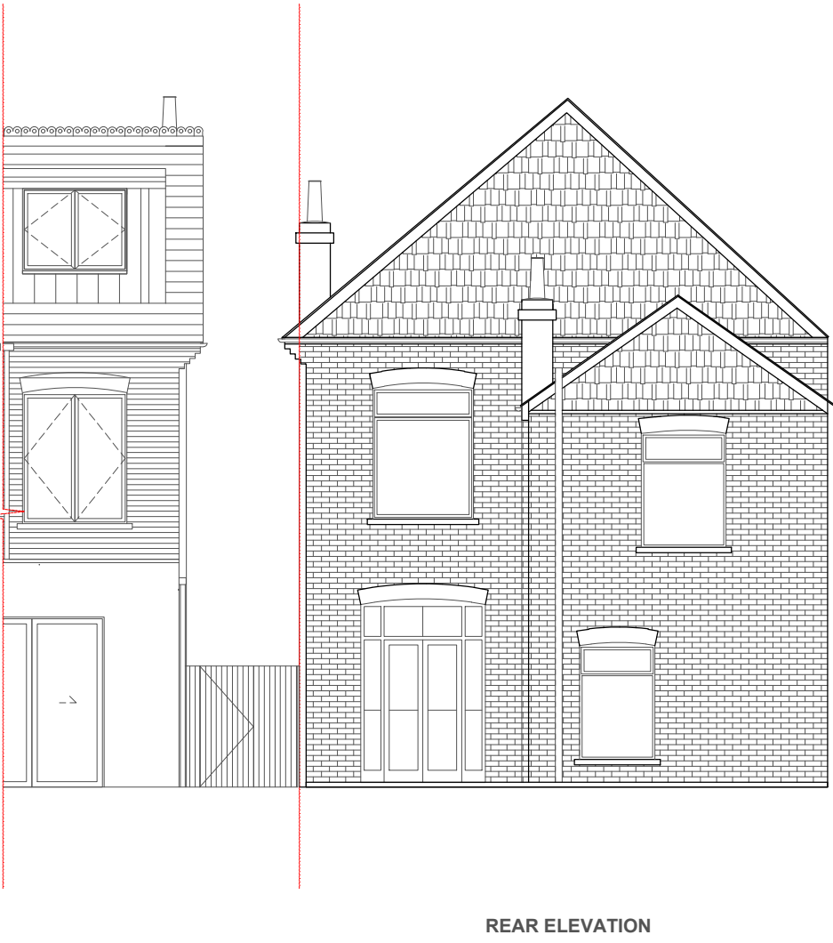
REAR ELEVATION
