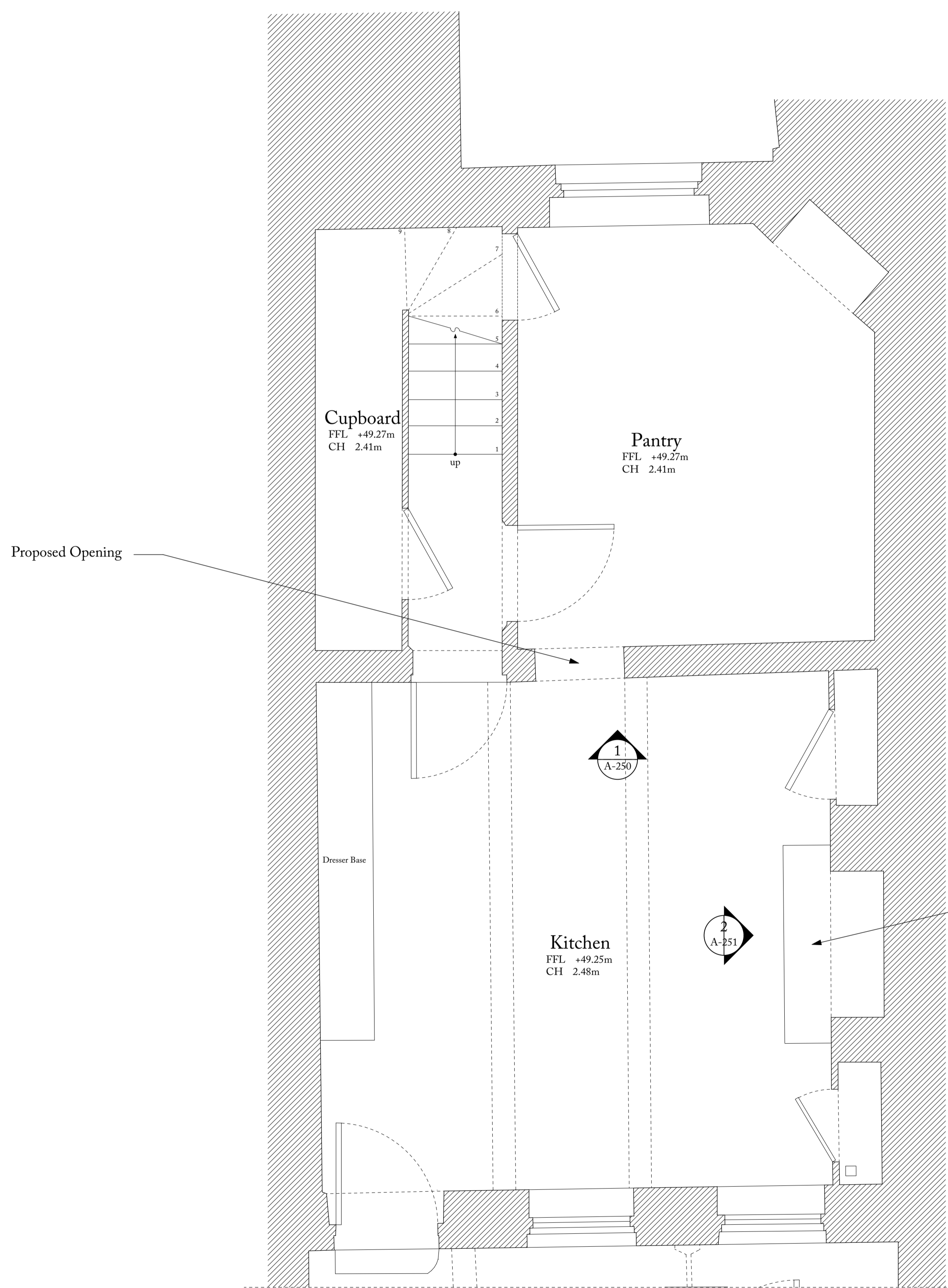
1 LOWER GROUND FLOOR PLAN 1:25 @ A1 / 1:50 @ A3
