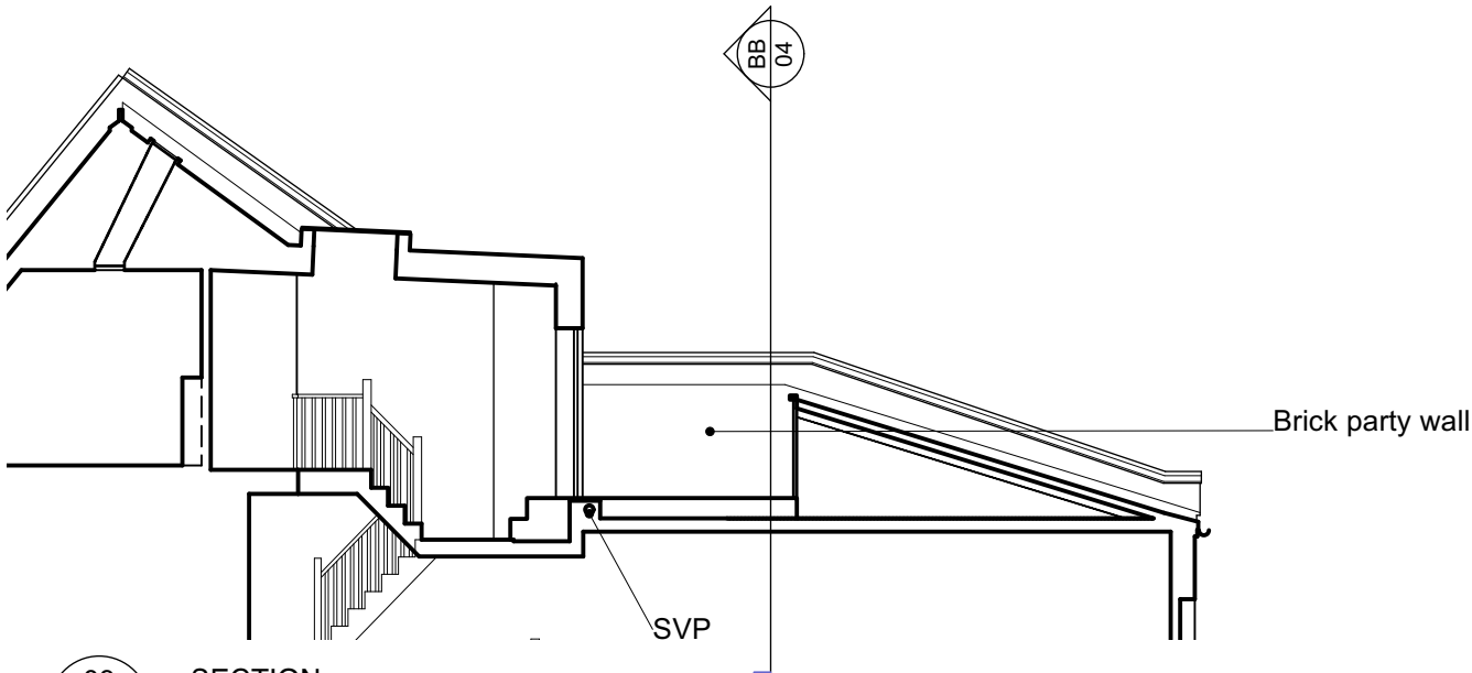
03 005 SECTION AA LONG
