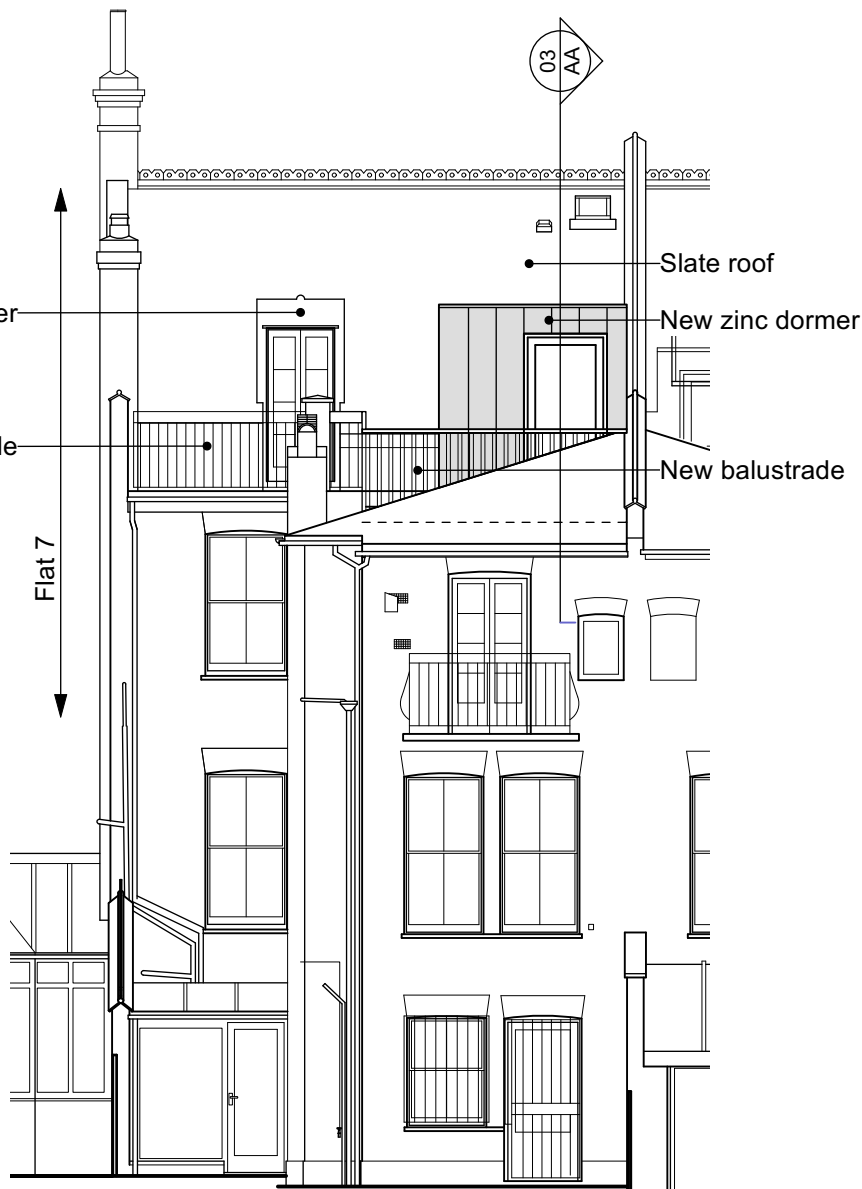
02 005 ELEVATION REAR
