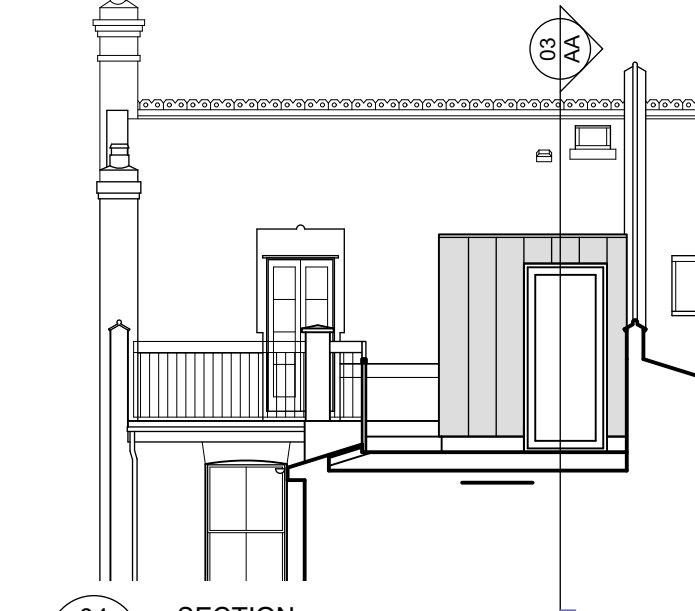
04 005 SECTION BB SHORT
