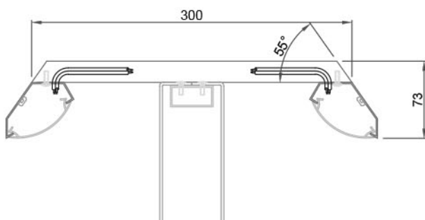
TYP front elevation section thru projection sign trough light
