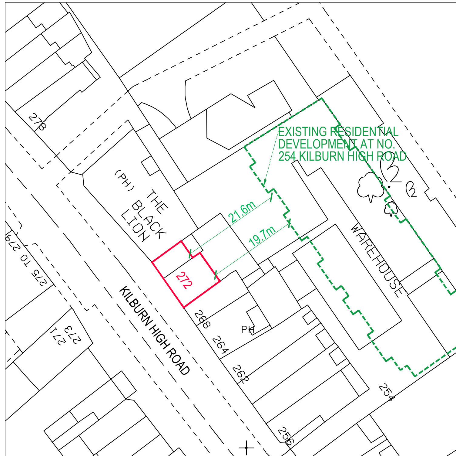
BLOCK PLAN scale 1:500 0 10 20 30m scale 1:500
