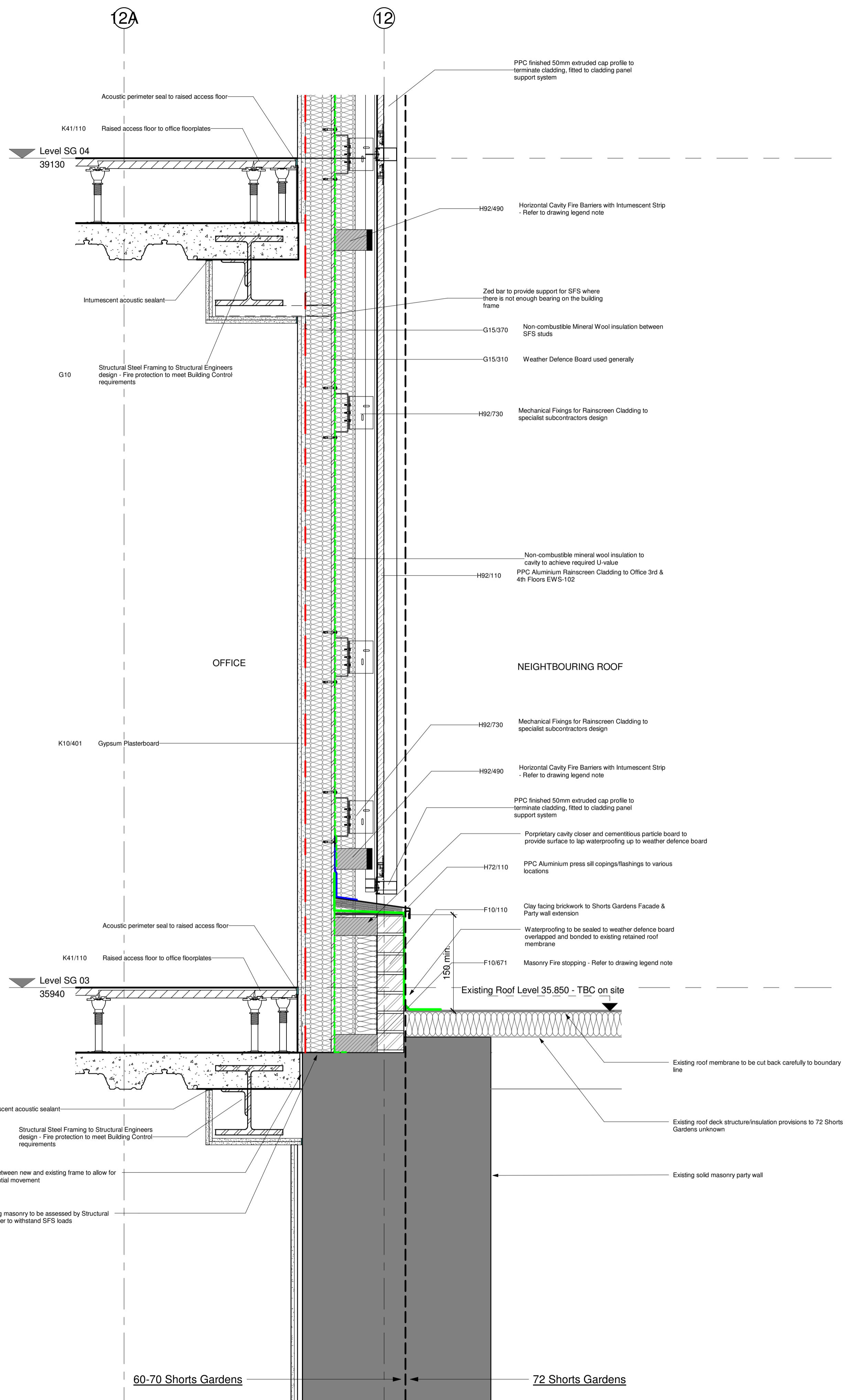
1 East Facade - Party Wall Cladding Interface - Section Detail 1 1 : 10
