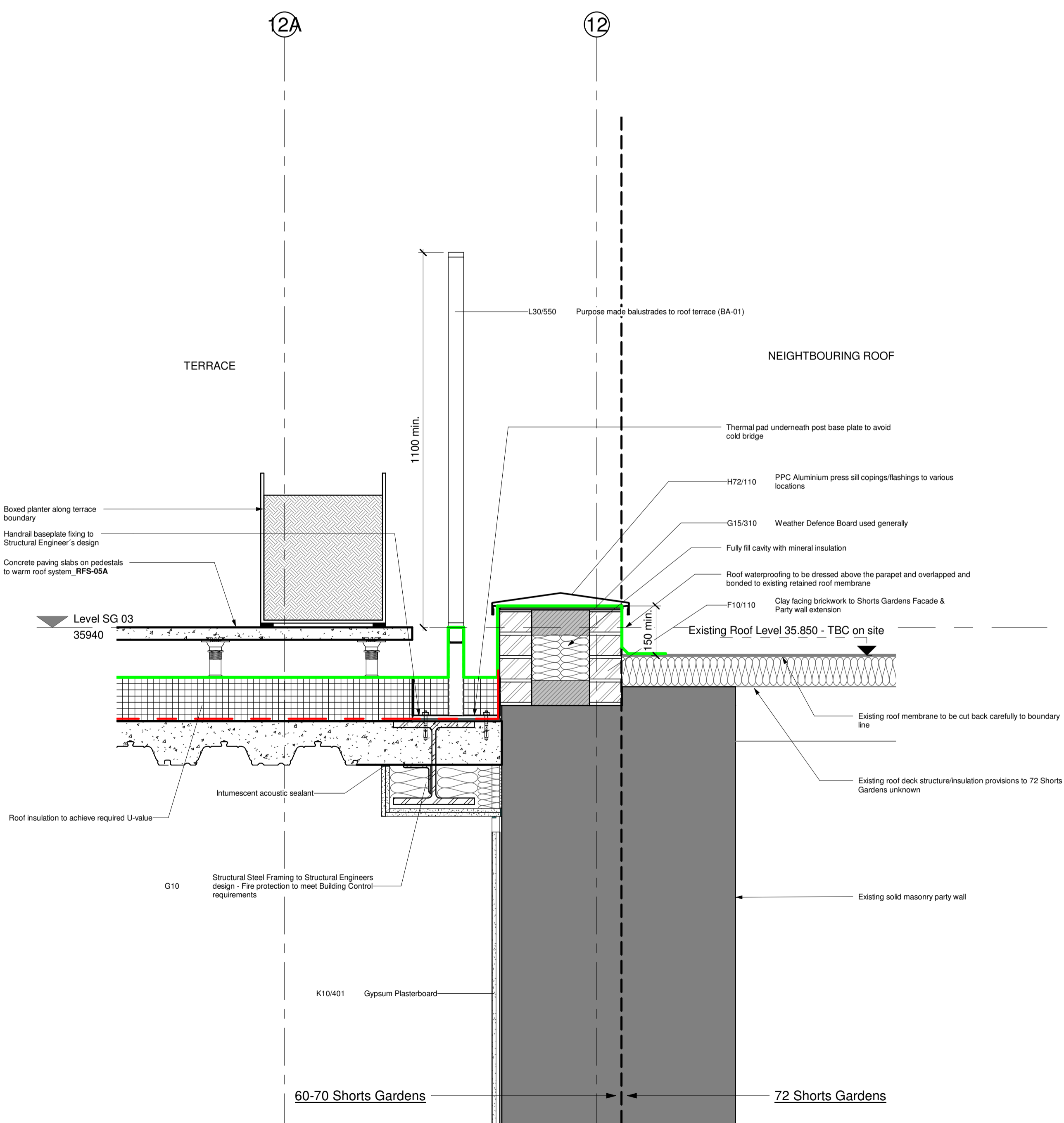
2 East facade - Party Wall Coping Interface - Section Detail 2 1 : 10
