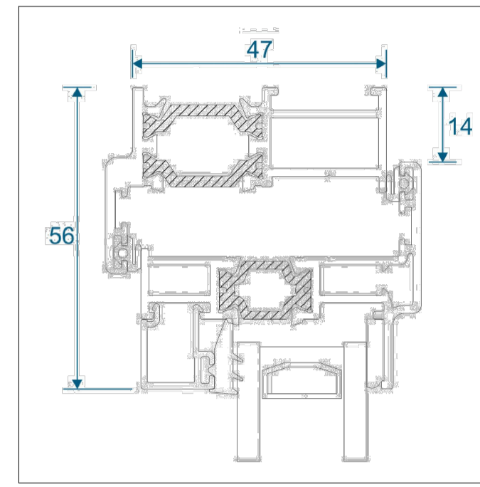
Section F-F Opener
