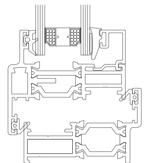
Section 34
