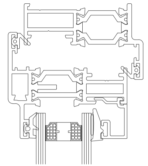
Section 32
