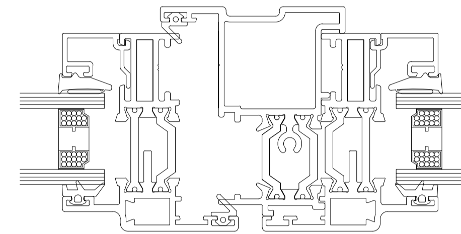
Section 36
