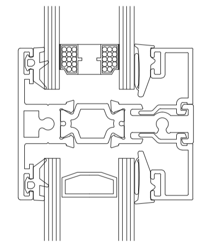
Section 34
