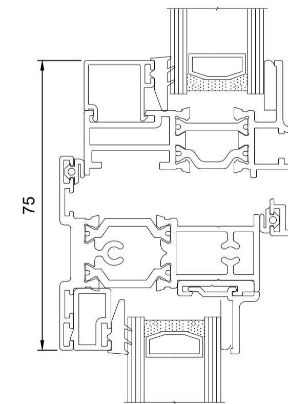
Section K-K
