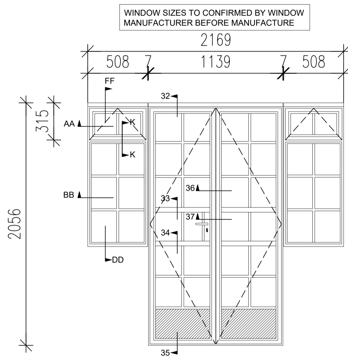
PROPOSED WINDOW/FRENCH DOOR - SCALE 1:20 MANUFACTURED BY DURATION WINDOWS
