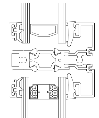
Section 33
