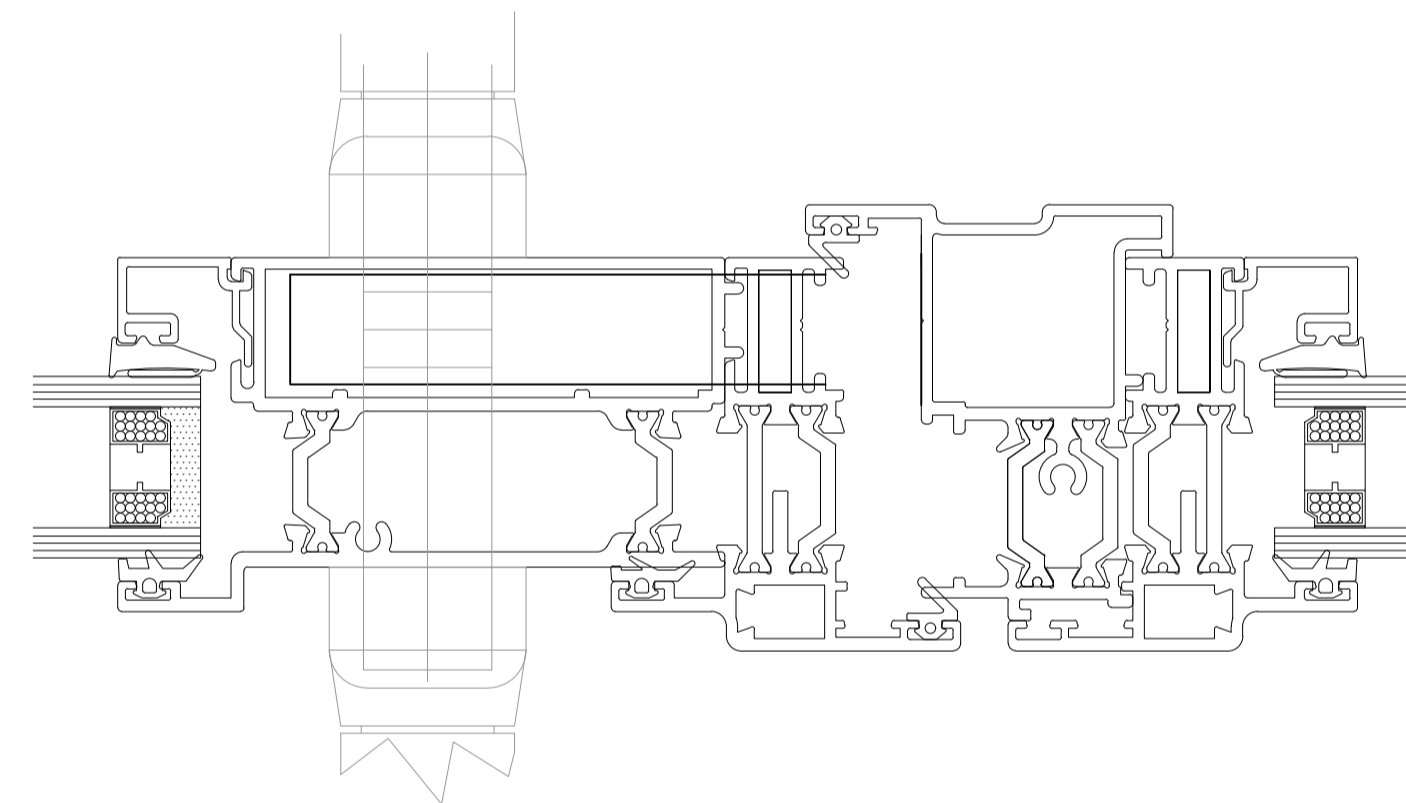
Section 37
