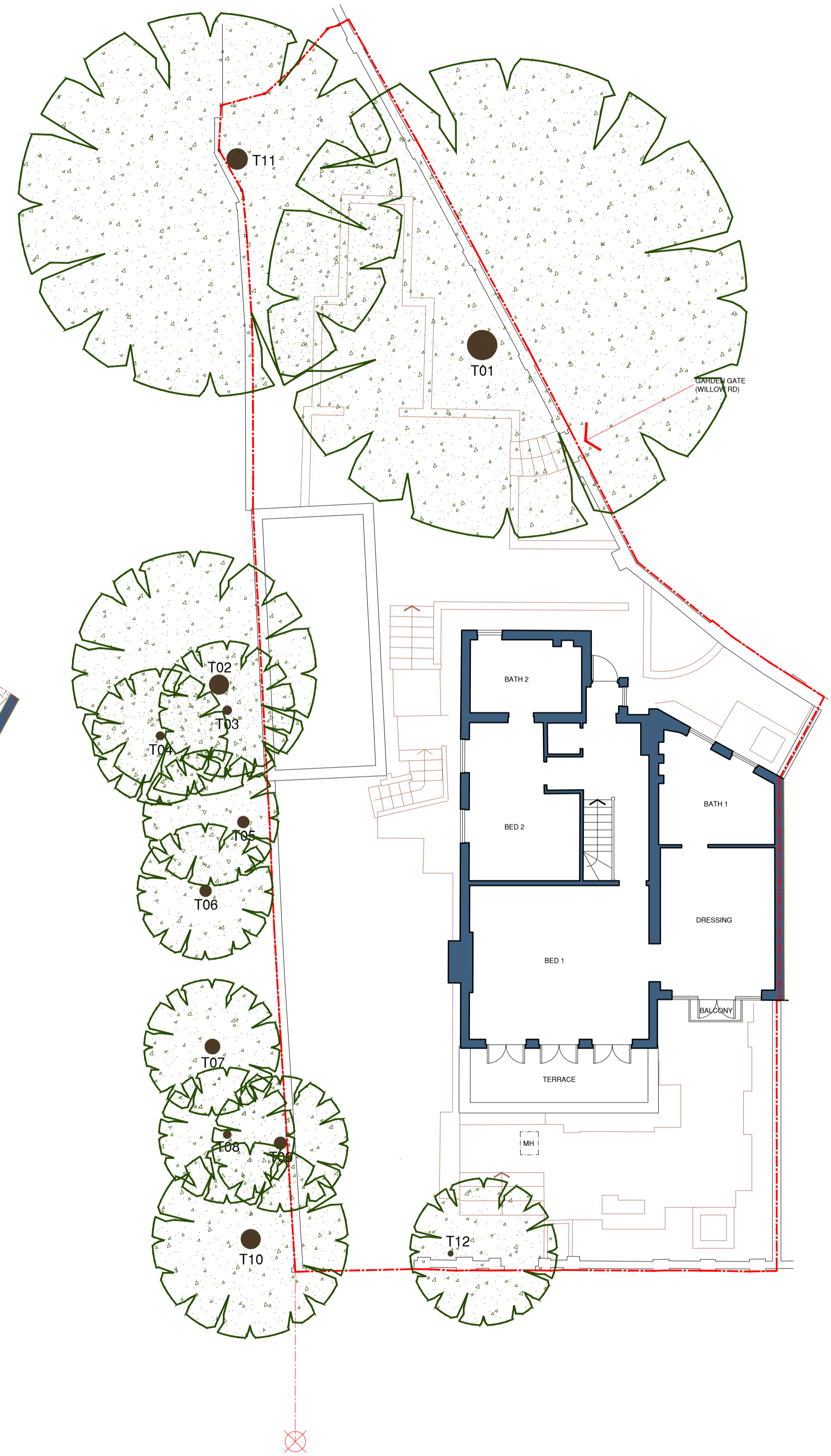
FIRST FLOOR
