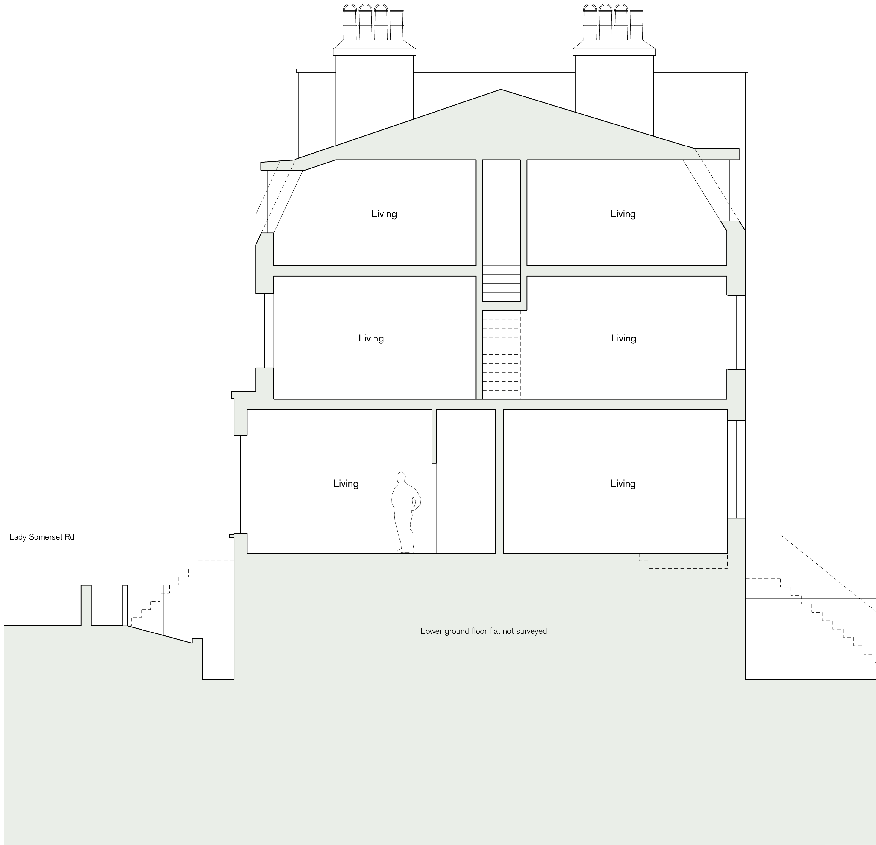
Section A
