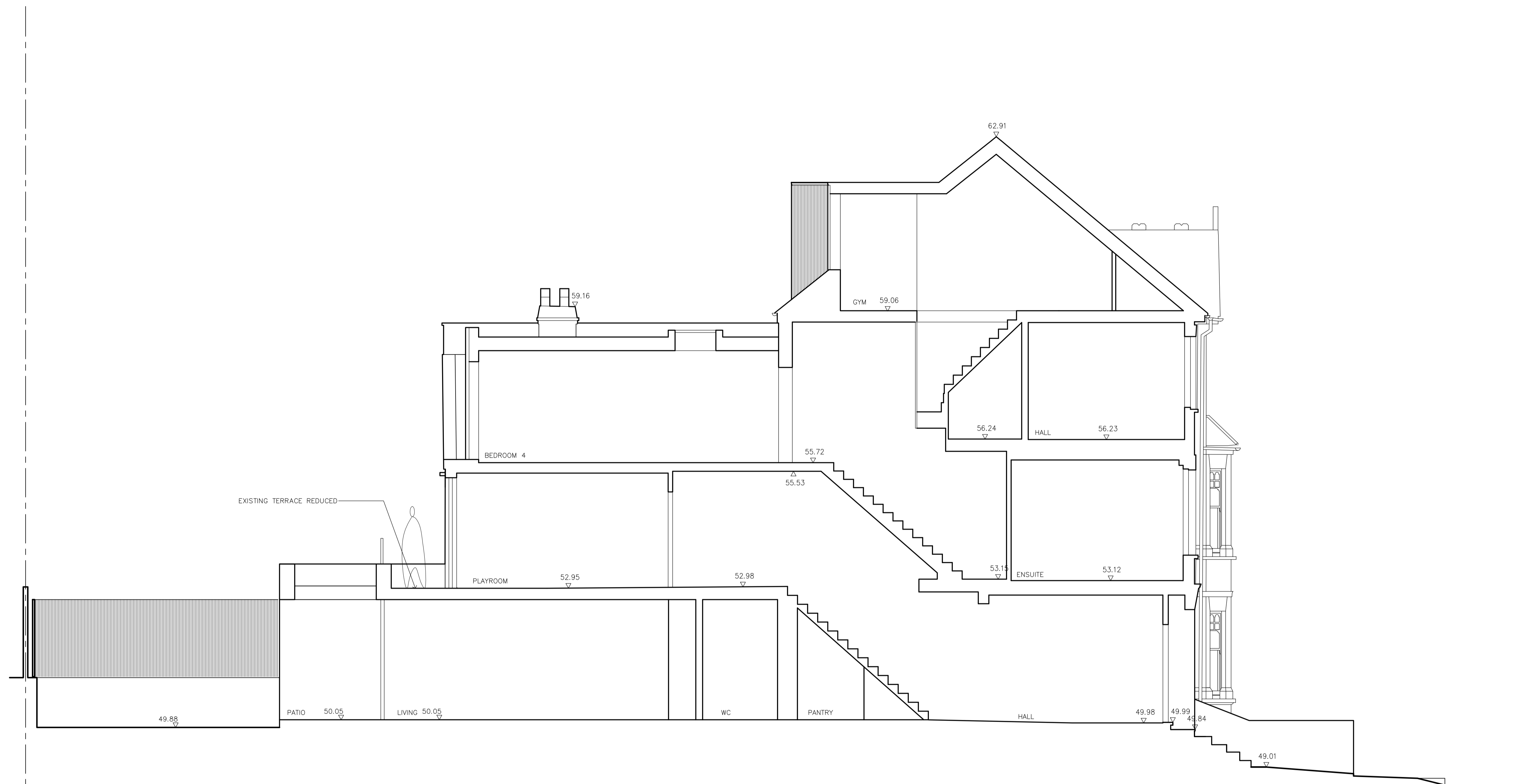
SECTION AA
