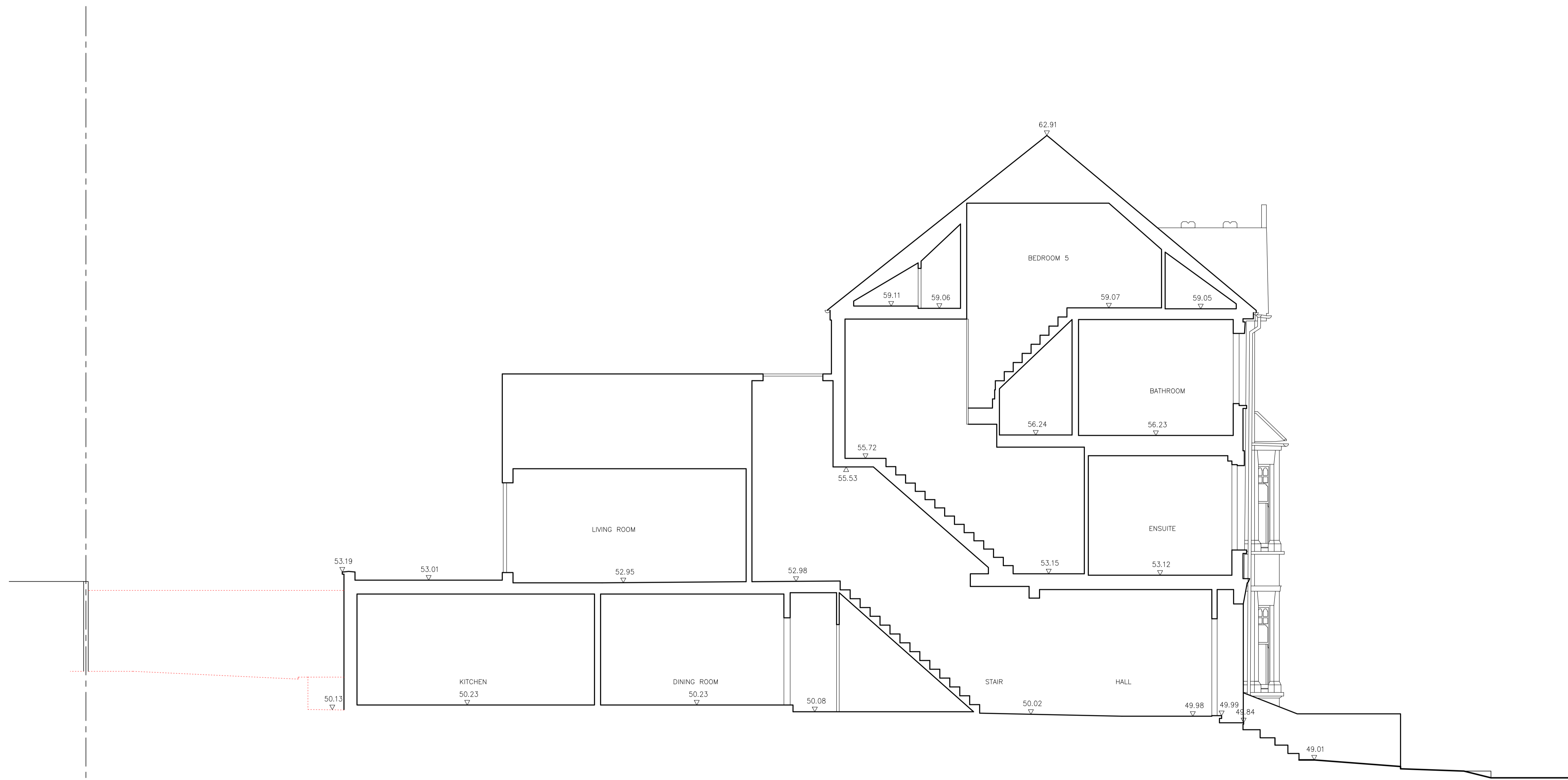
SECTION AA
