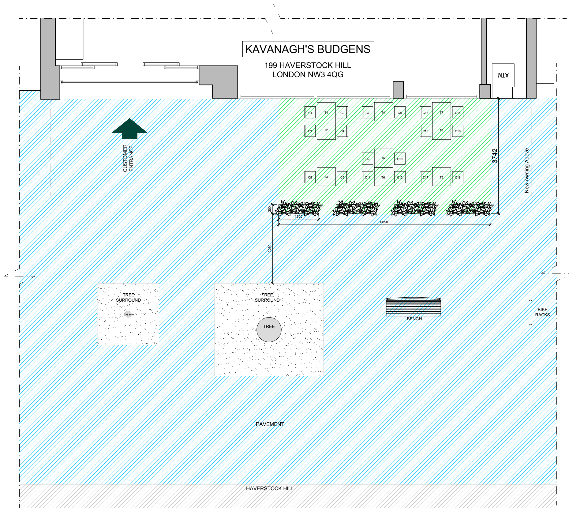
PROPOSED SEATING AND PAVEMENT PLAN
