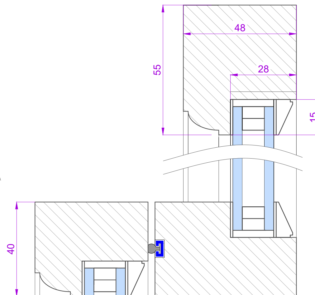
SECTION THROUGH HEAD RAIL, MEETING RAIL & BOTTOM RAIL - SCALE 1:1
