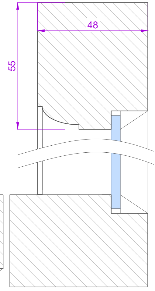
SECTION THROUGH HEAD RAIL, MEETING RAIL & BOTTOM RAIL - SCALE 1:1
