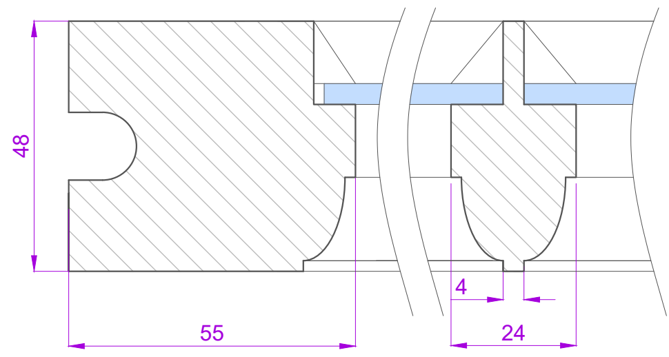
SECTION THROUGH STILE & GLAZING BAR - SCALE 1:1
