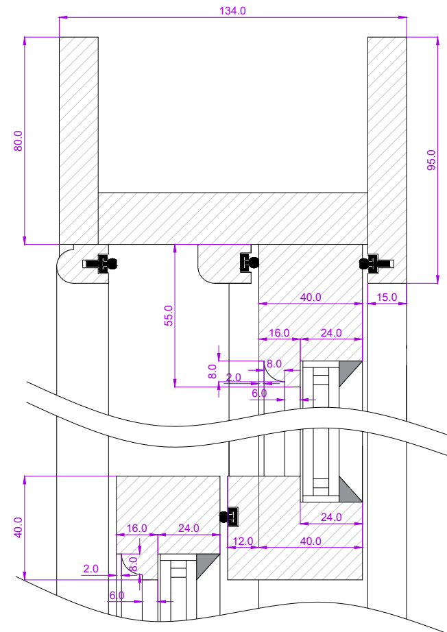
FRAME / SASH HEAD DETAILS
