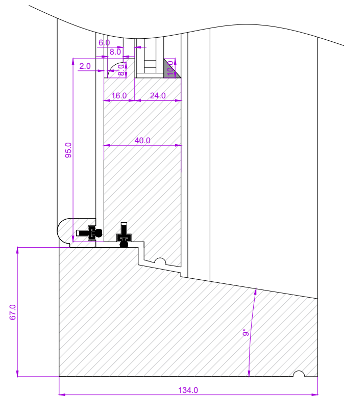
BOTTOM RAIL / CILL DETAILS
