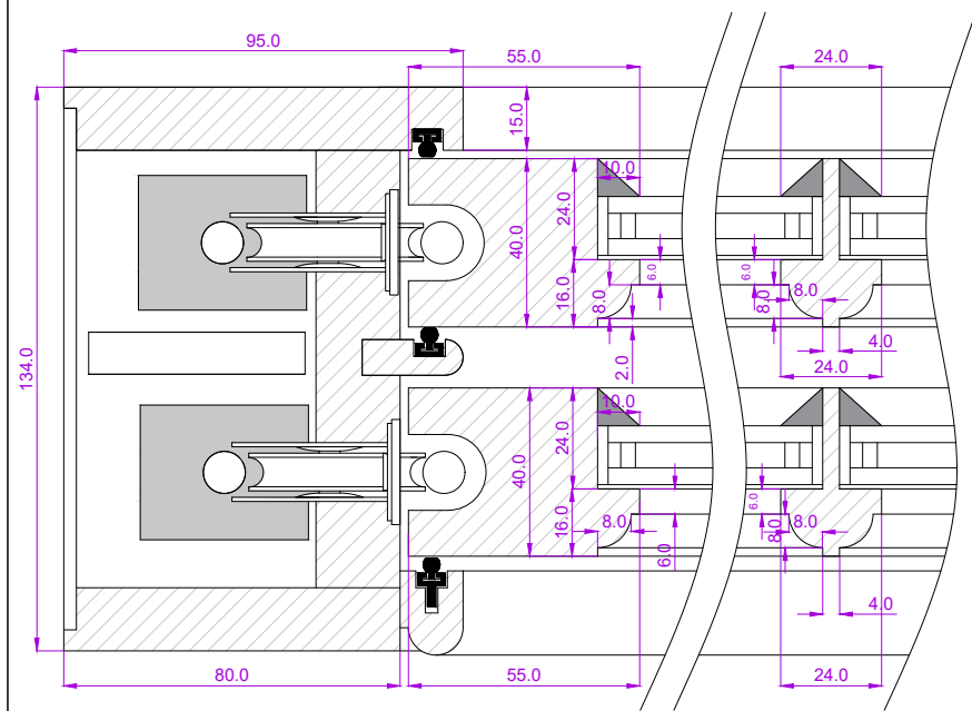
GLAZING BAR DETAILS
