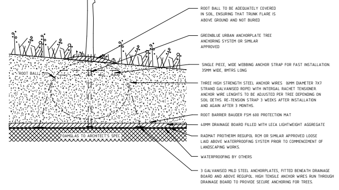
DETAILS TREE ANCHORING SYSTEM - FOR ALL TREES ON 1ST AND 10TH FLOOR SCALE 1:10
