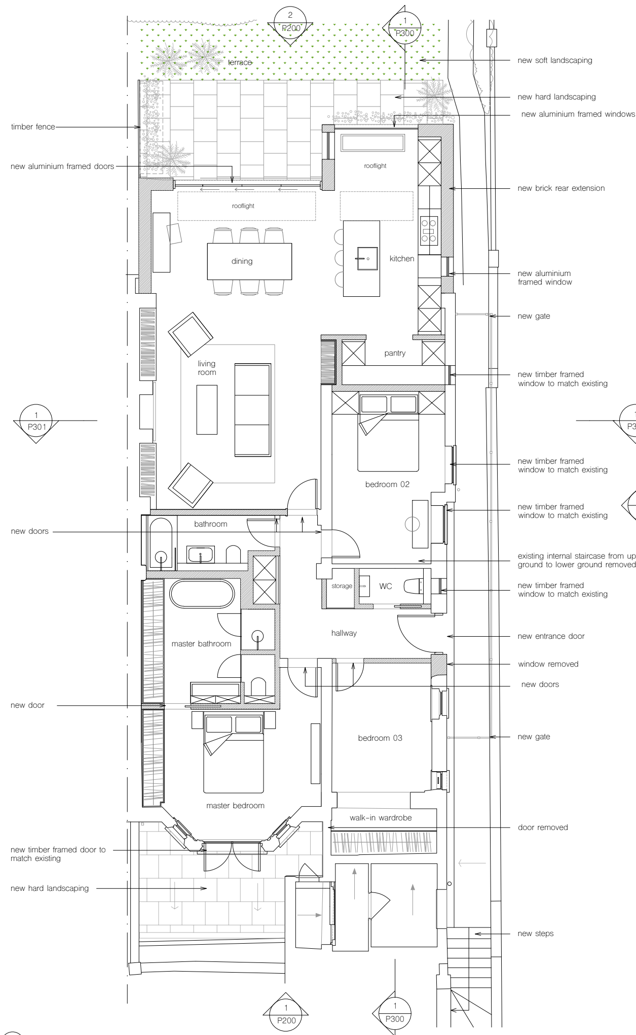
1 lower ground floor plan
