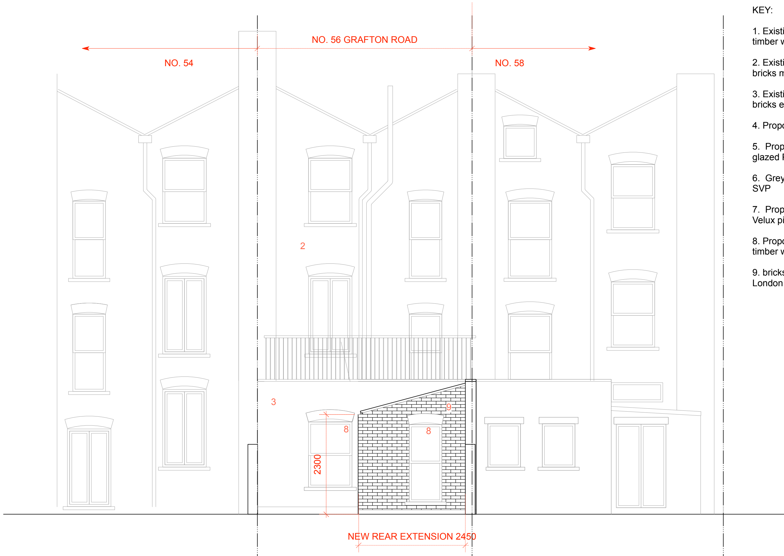
PROPOSED Rear Elevation AA
