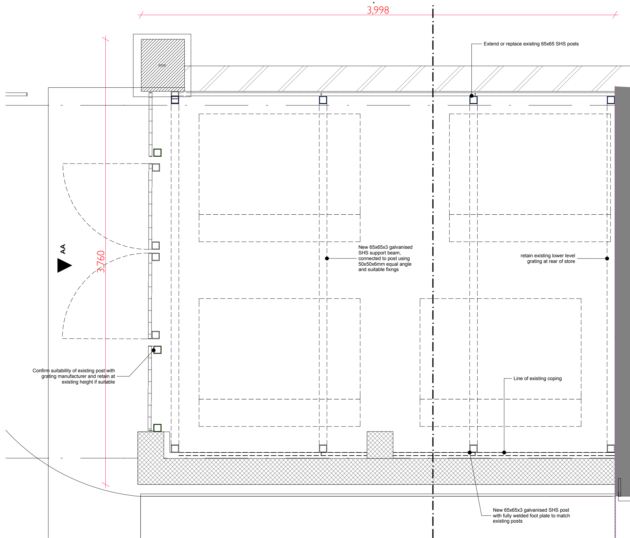
Refuse store plan 1:20
