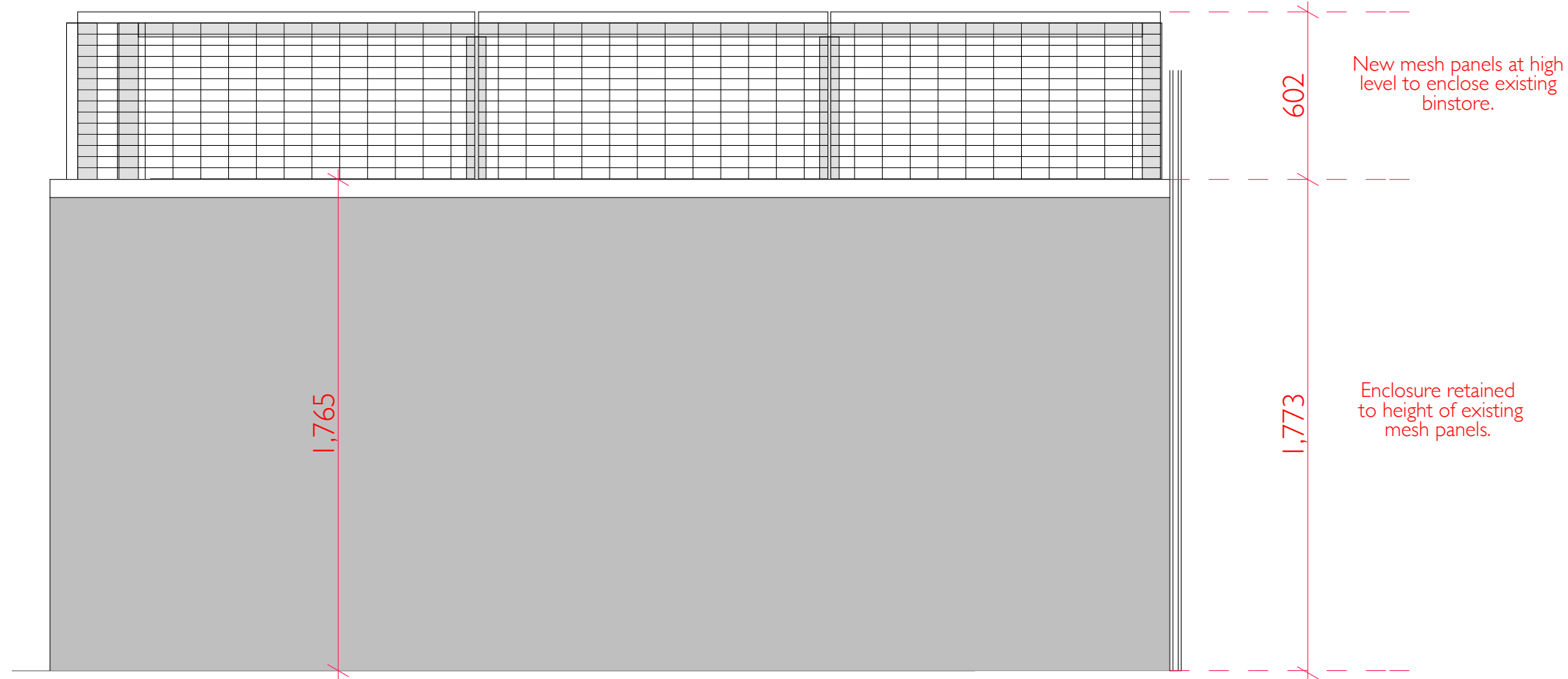
Proposed Elevation B-B 1:20
