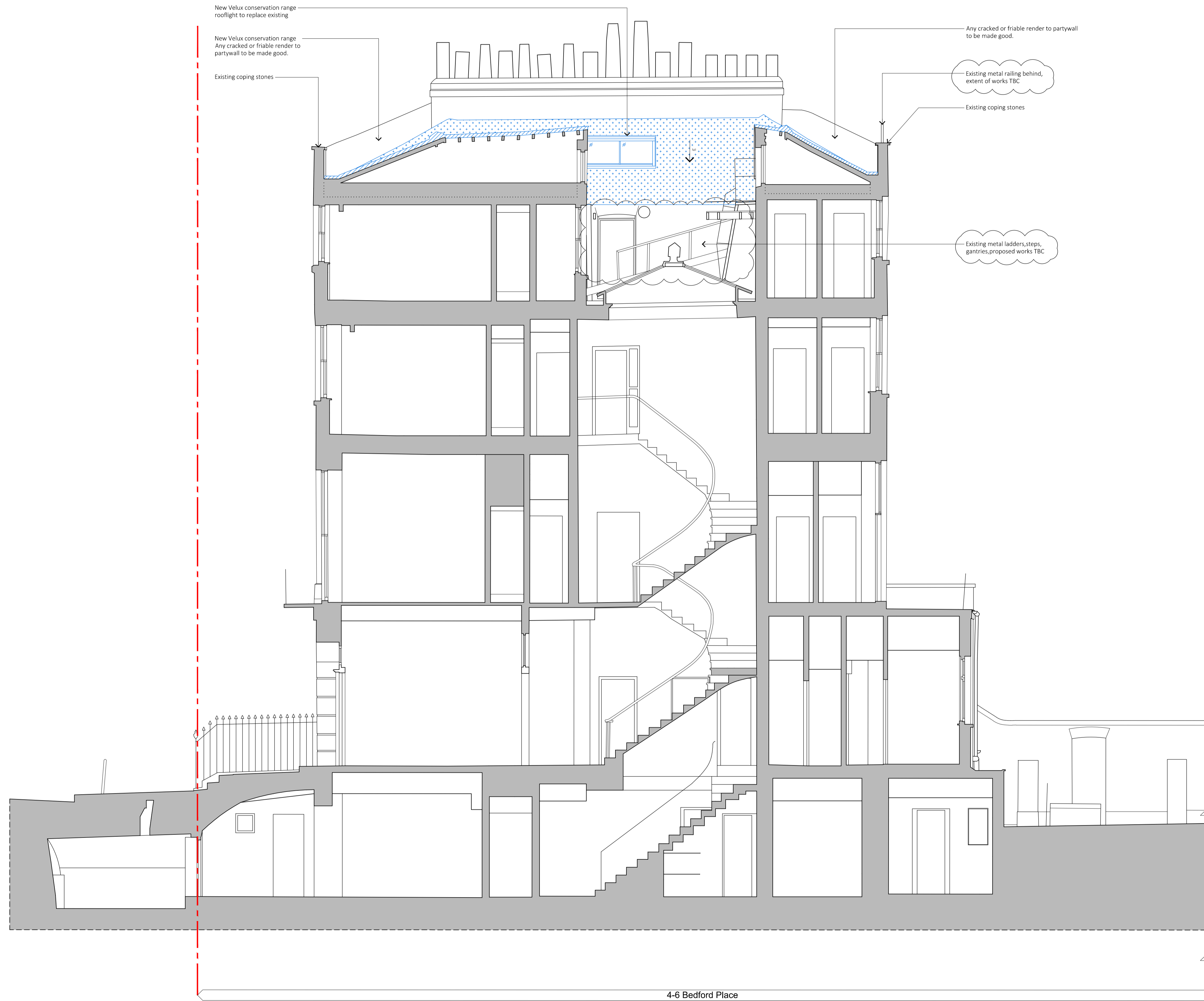
1 Proposed Section A-A 1:50 @ A1
